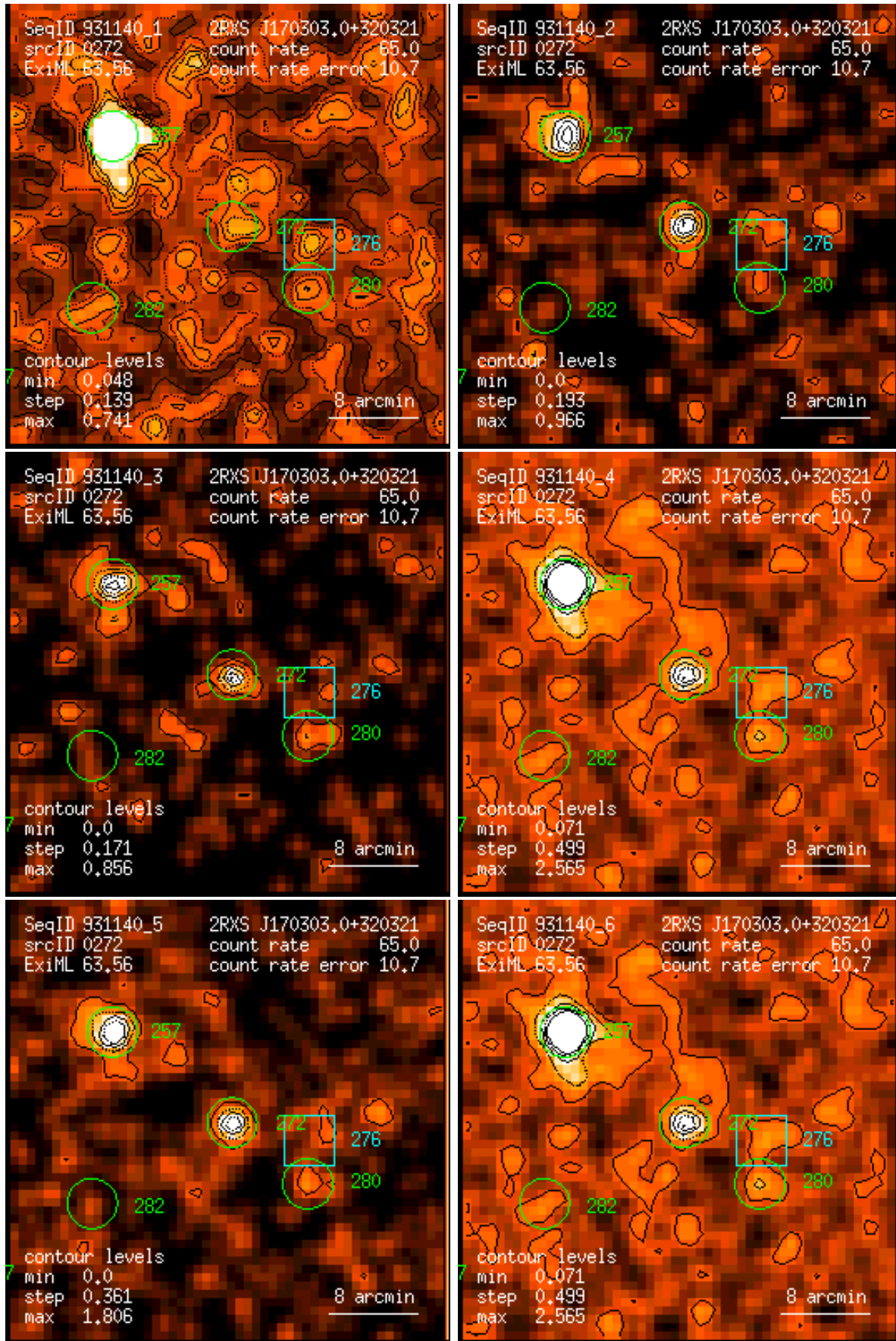
Figure 272: RASS 931140: detection 0272: band rate images, Gaussian filter: (1) PSPC channels 11 – 41, (2) 52 – 90, (3) 91 – 201, (4) 11 – 235, (5) 52 – 201, (6) 11 – 201. Broad band rates in counts/ks. Band rate contour levels in counts/ks/arcmin 2 .
