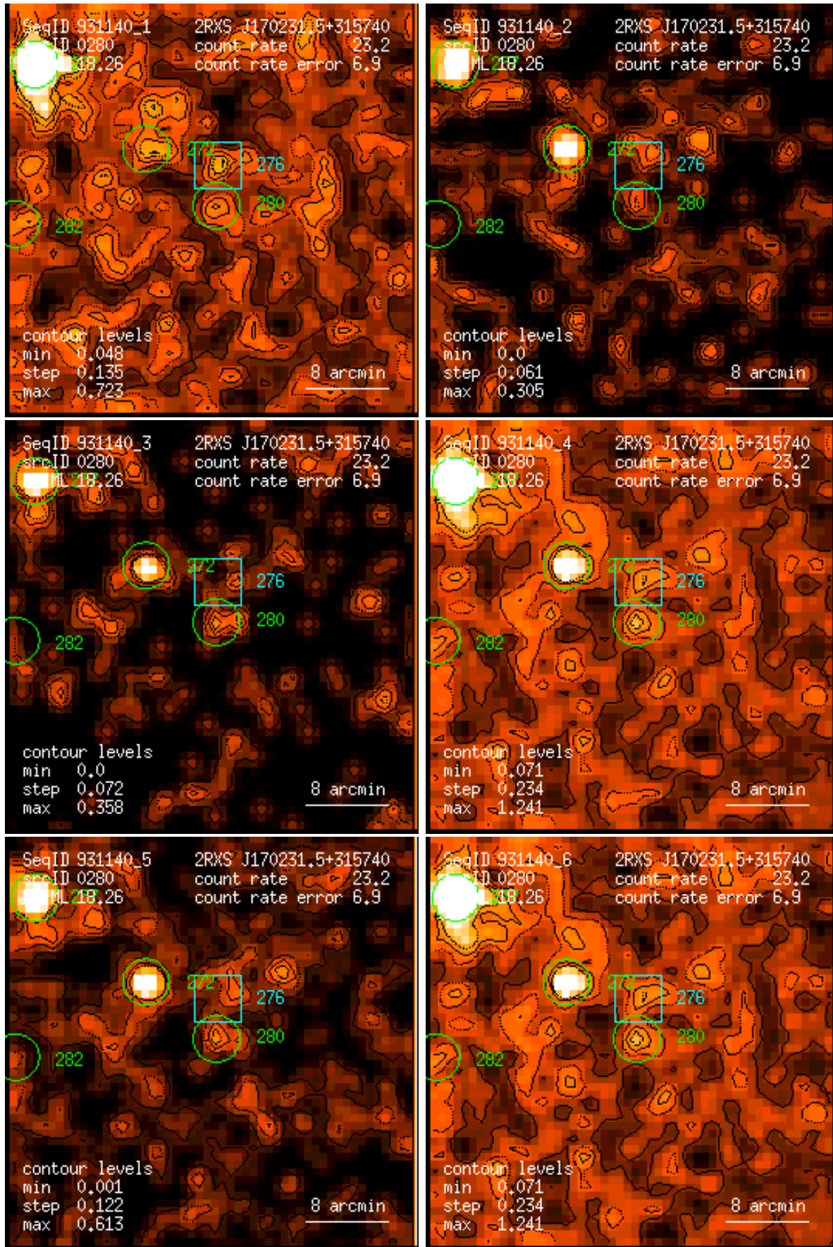
Figure 280: RASS 931140: detection 0280: band rate images, Gaussian filter: (1) PSPC channels 11 – 41, (2) 52 – 90, (3) 91 – 201, (4) 11 – 235, (5) 52 – 201, (6) 11 – 201. Broad band rates in counts/ks. Band rate contour levels in counts/ks/arcmin 2 .
