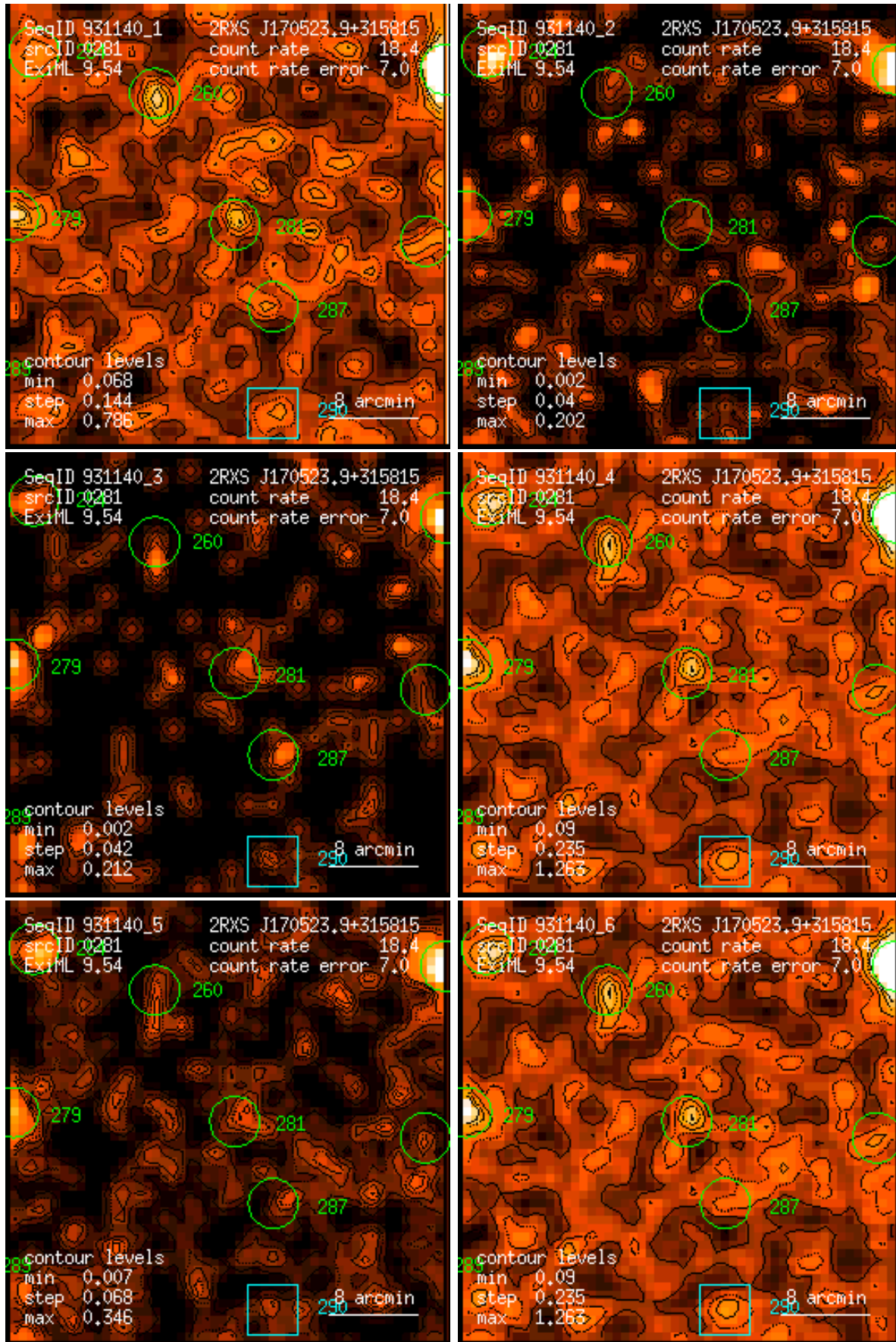
Figure 281: RASS 931140: detection 0281: band rate images, Gaussian filter: (1) PSPC channels 11 – 41, (2) 52 – 90, (3) 91 – 201, (4) 11 – 235, (5) 52 – 201, (6) 11 – 201. Broad band rates in counts/ks. Band rate contour levels in counts/ks/arcmin 2 .
