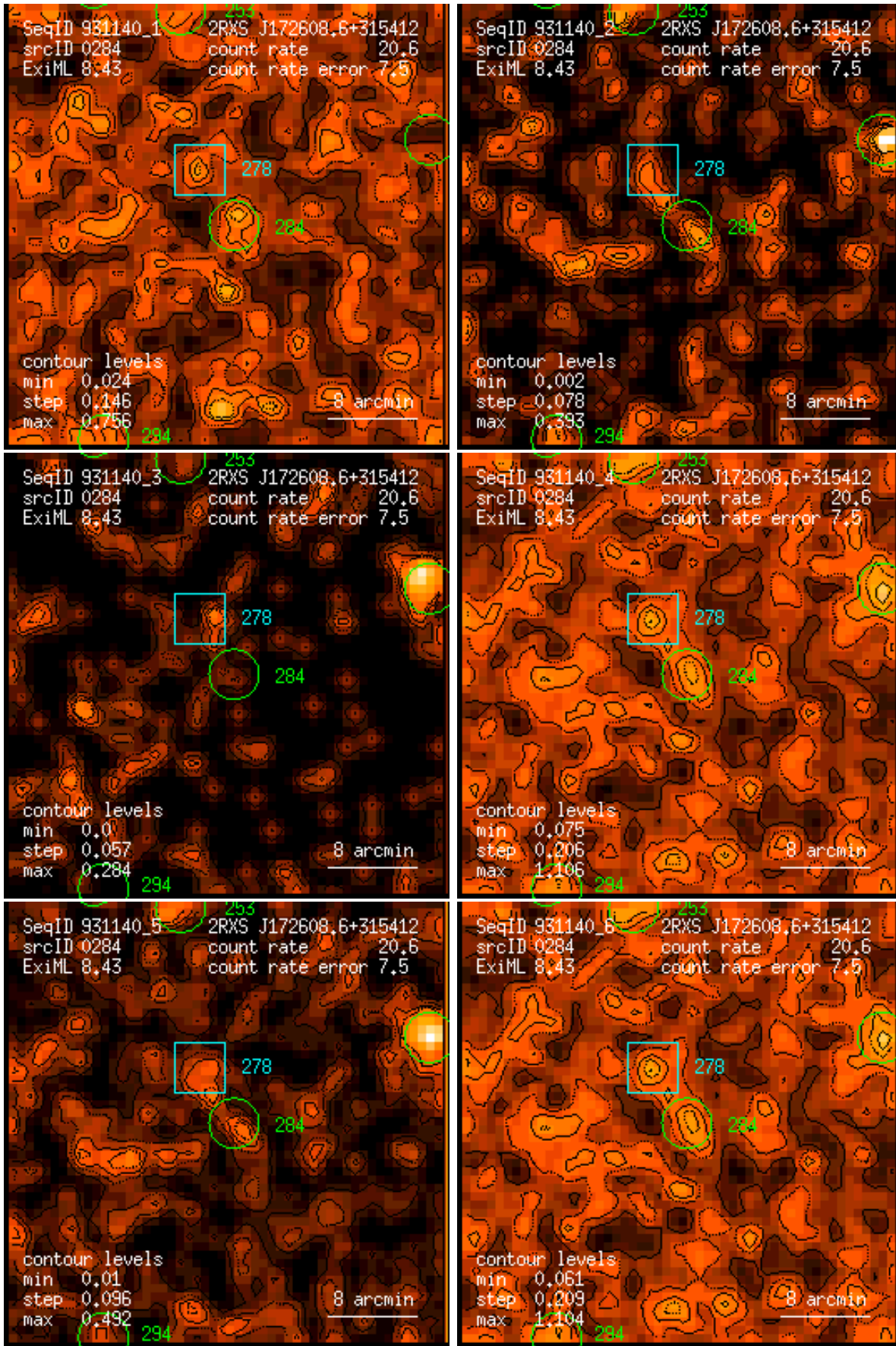
Figure 284: RASS 931140: detection 0284: band rate images, Gaussian filter: (1) PSPC channels 11 – 41, (2) 52 – 90, (3) 91 – 201, (4) 11 – 235, (5) 52 – 201, (6) 11 – 201. Broad band rates in counts/ks. Band rate contour levels in counts/ks/arcmin 2 .
