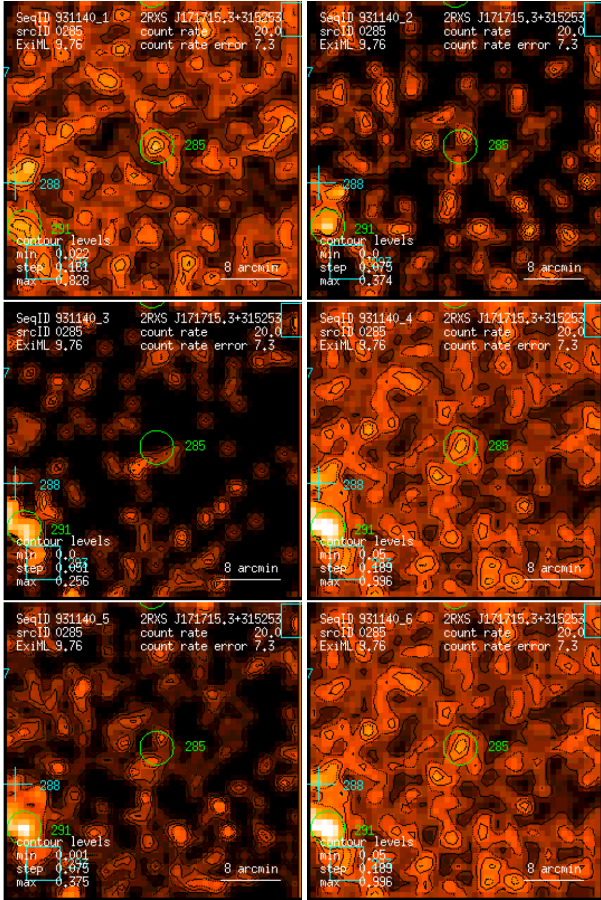
Figure 285: RASS 931140: detection 0285: band rate images, Gaussian filter: (1) PSPC channels 11 – 41, (2) 52 – 90, (3) 91 – 201, (4) 11 – 235, (5) 52 – 201, (6) 11 – 201. Broad band rates in counts/ks. Band rate contour levels in counts/ks/arcmin 2 .
