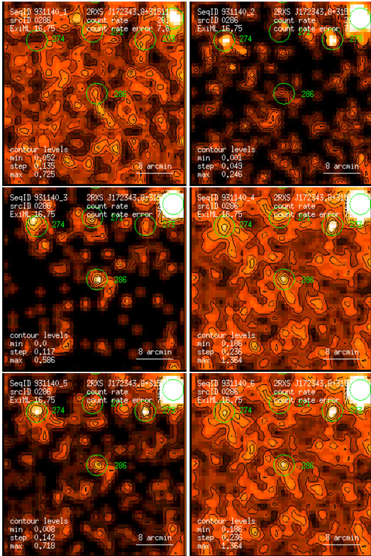
Figure 286: RASS 931140: detection 0286: band rate images, Gaussian filter: (1) PSPC channels 11 – 41, (2) 52 – 90, (3) 91 – 201, (4) 11 – 235, (5) 52 – 201, (6) 11 – 201. Broad band rates in counts/ks. Band rate contour levels in counts/ks/arcmin 2 .
