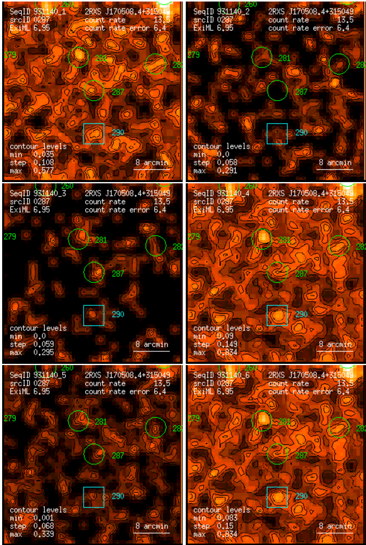
Figure 287: RASS 931140: detection 0287: band rate images, Gaussian filter: (1) PSPC channels 11 – 41, (2) 52 – 90, (3) 91 – 201, (4) 11 – 235, (5) 52 – 201, (6) 11 – 201. Broad band rates in counts/ks. Band rate contour levels in counts/ks/arcmin 2 .
