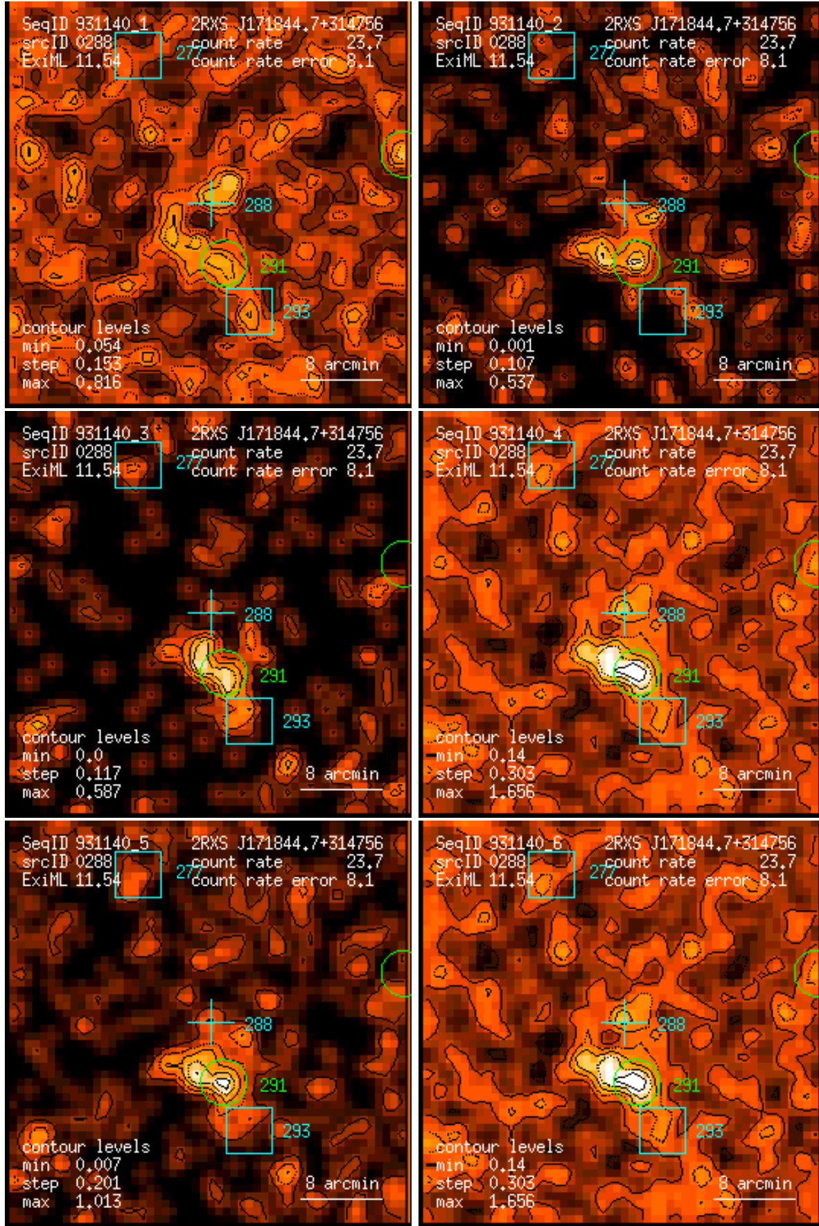
Figure 288: RASS 931140: detection 0288: band rate images, Gaussian filter: (1) PSPC channels 11 – 41, (2) 52 – 90, (3) 91 – 201, (4) 11 – 235, (5) 52 – 201, (6) 11 – 201. Broad band rates in counts/ks. Band rate contour levels in counts/ks/arcmin 2 .
