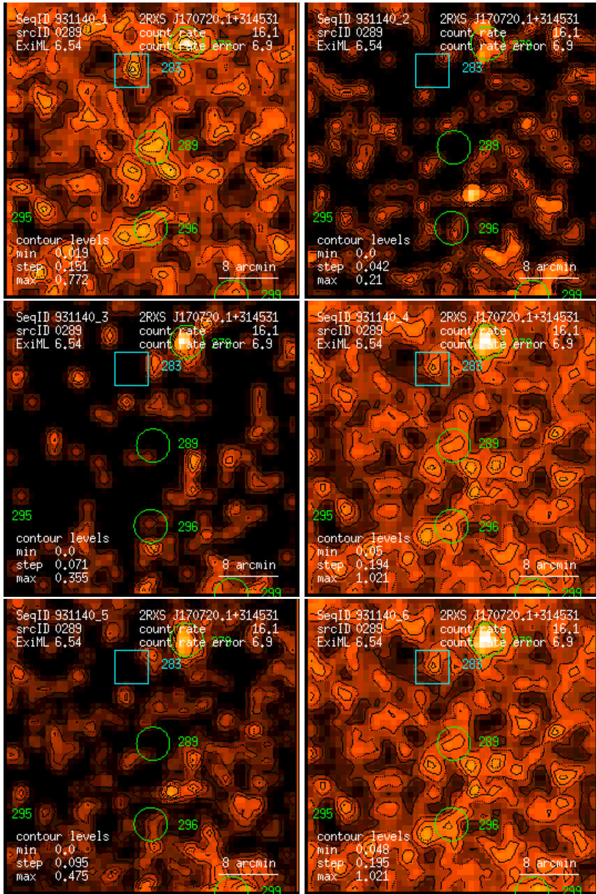
Figure 289: RASS 931140: detection 0289: band rate images, Gaussian filter: (1) PSPC channels 11 – 41, (2) 52 – 90, (3) 91 – 201, (4) 11 – 235, (5) 52 – 201, (6) 11 – 201. Broad band rates in counts/ks. Band rate contour levels in counts/ks/arcmin 2 .
