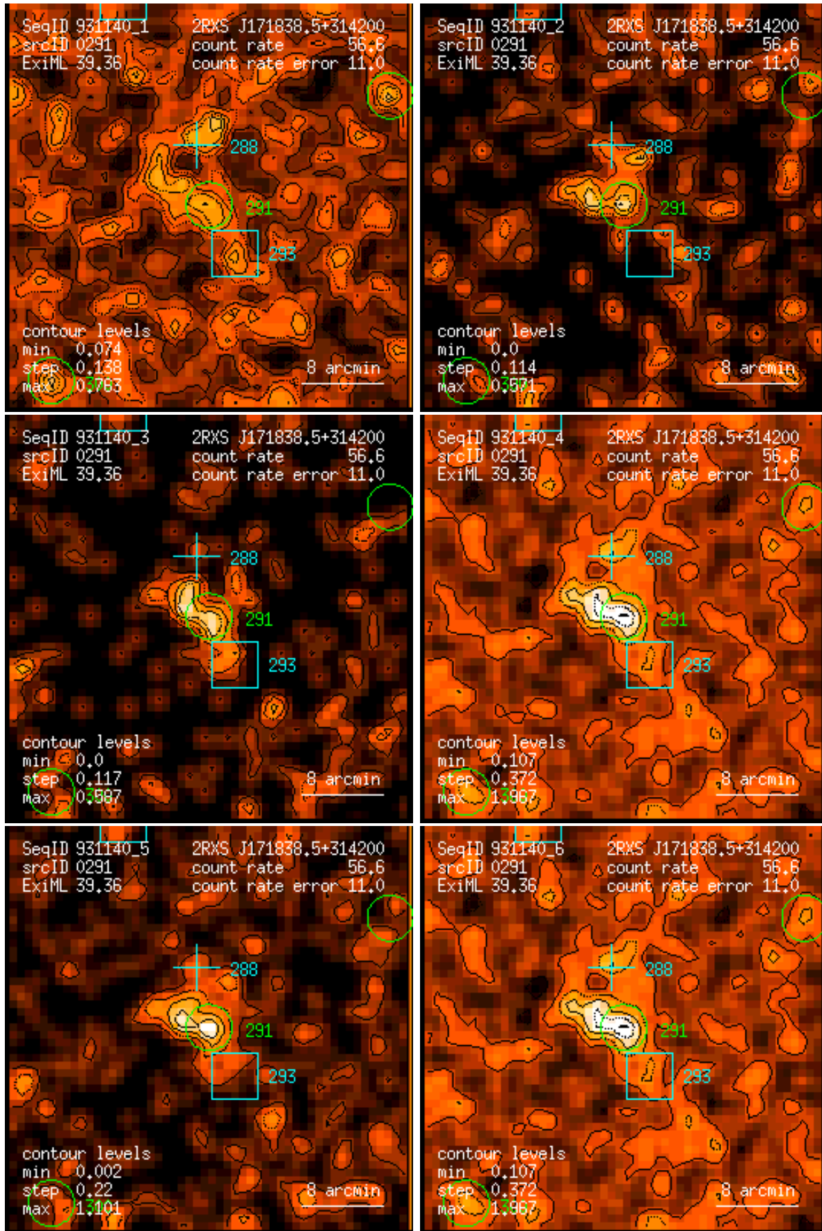
Figure 291: RASS 931140: detection 0291: band rate images, Gaussian filter: (1) PSPC channels 11 – 41, (2) 52 – 90, (3) 91 – 201, (4) 11 – 235, (5) 52 – 201, (6) 11 – 201. Broad band rates in counts/ks. Band rate contour levels in counts/ks/arcmin 2 .
