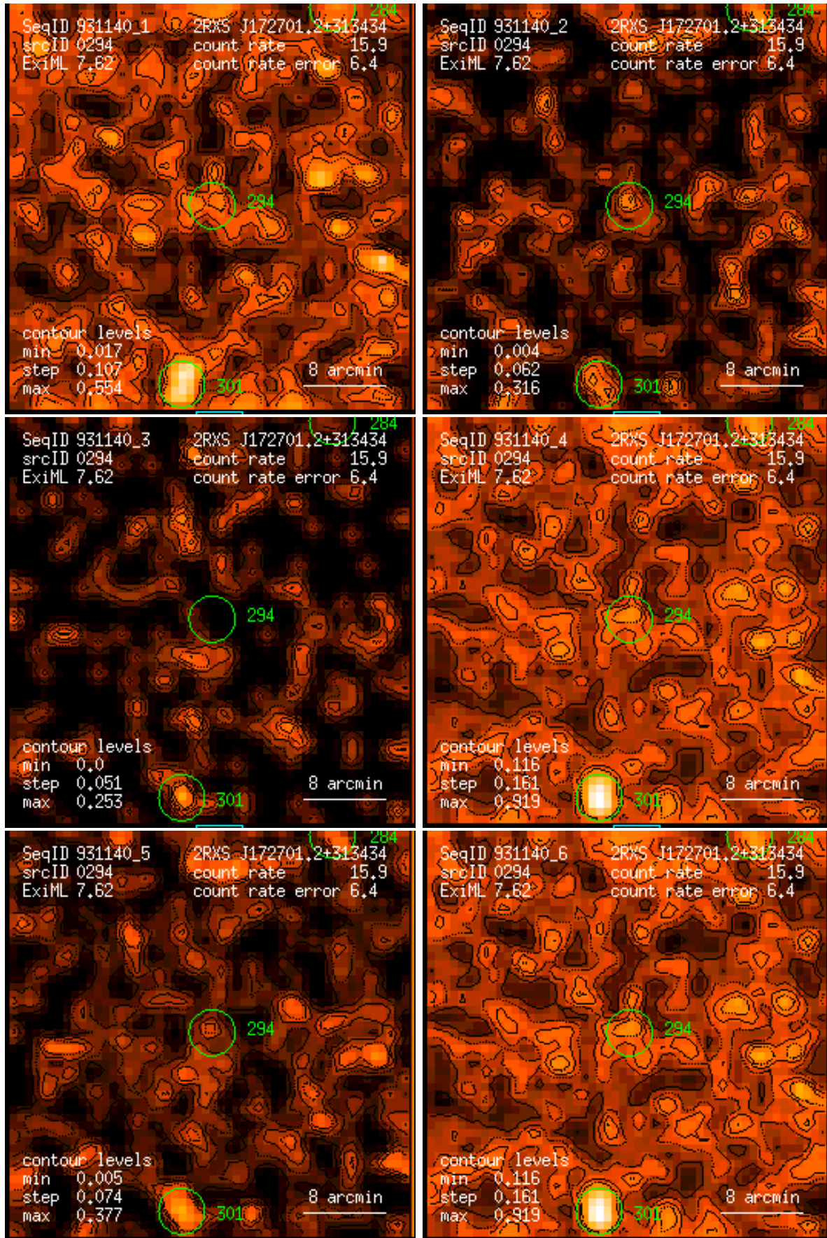
Figure 294: RASS 931140: detection 0294: band rate images, Gaussian filter: (1) PSPC channels 11 – 41, (2) 52 – 90, (3) 91 – 201, (4) 11 – 235, (5) 52 – 201, (6) 11 – 201. Broad band rates in counts/ks. Band rate contour levels in counts/ks/arcmin 2 .
