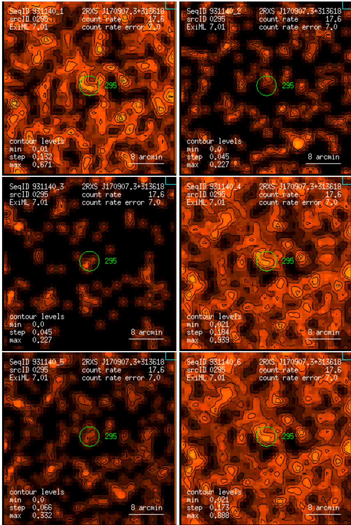
Figure 295: RASS 931140: detection 0295: band rate images, Gaussian filter: (1) PSPC channels 11 – 41, (2) 52 – 90, (3) 91 – 201, (4) 11 – 235, (5) 52 – 201, (6) 11 – 201. Broad band rates in counts/ks. Band rate contour levels in counts/ks/arcmin 2 .
