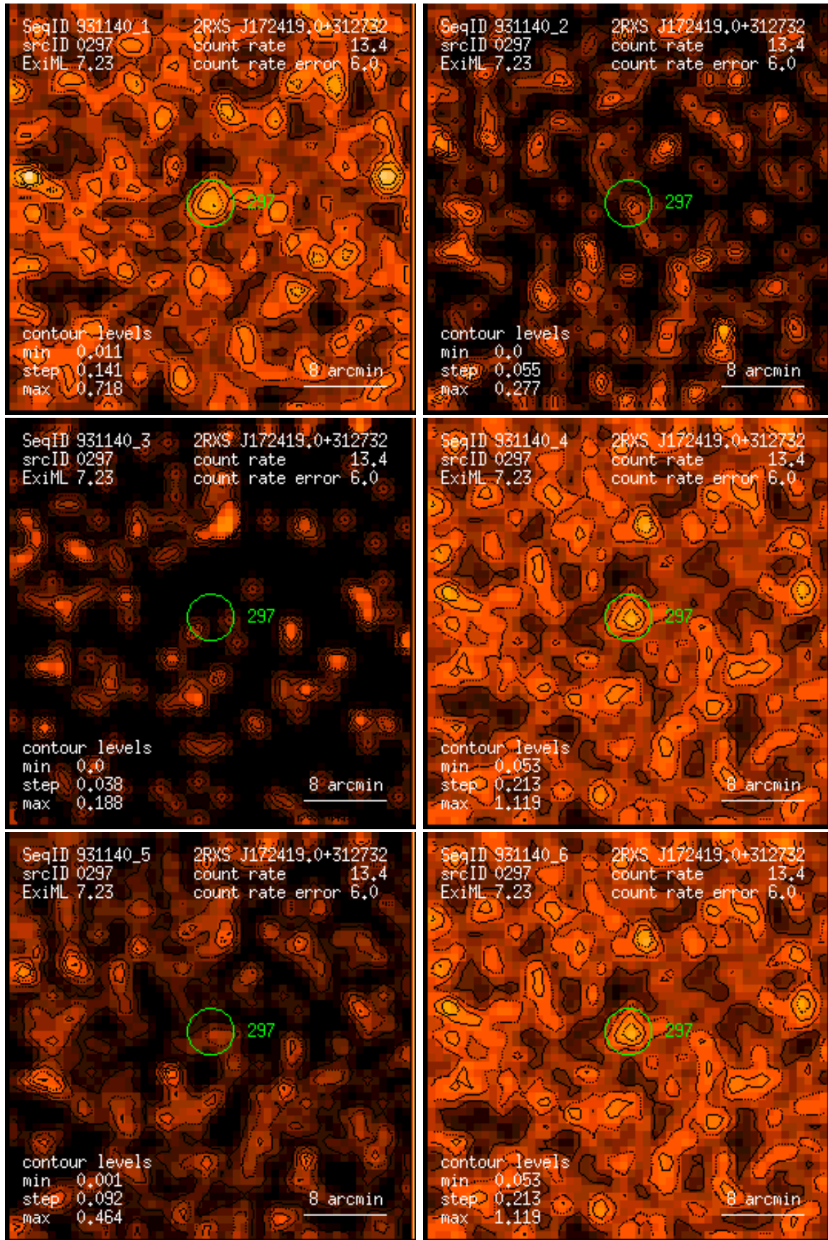
Figure 297: RASS 931140: detection 0297: band rate images, Gaussian filter: (1) PSPC channels 11 – 41, (2) 52 – 90, (3) 91 – 201, (4) 11 – 235, (5) 52 – 201, (6) 11 – 201. Broad band rates in counts/ks. Band rate contour levels in counts/ks/arcmin 2 .
