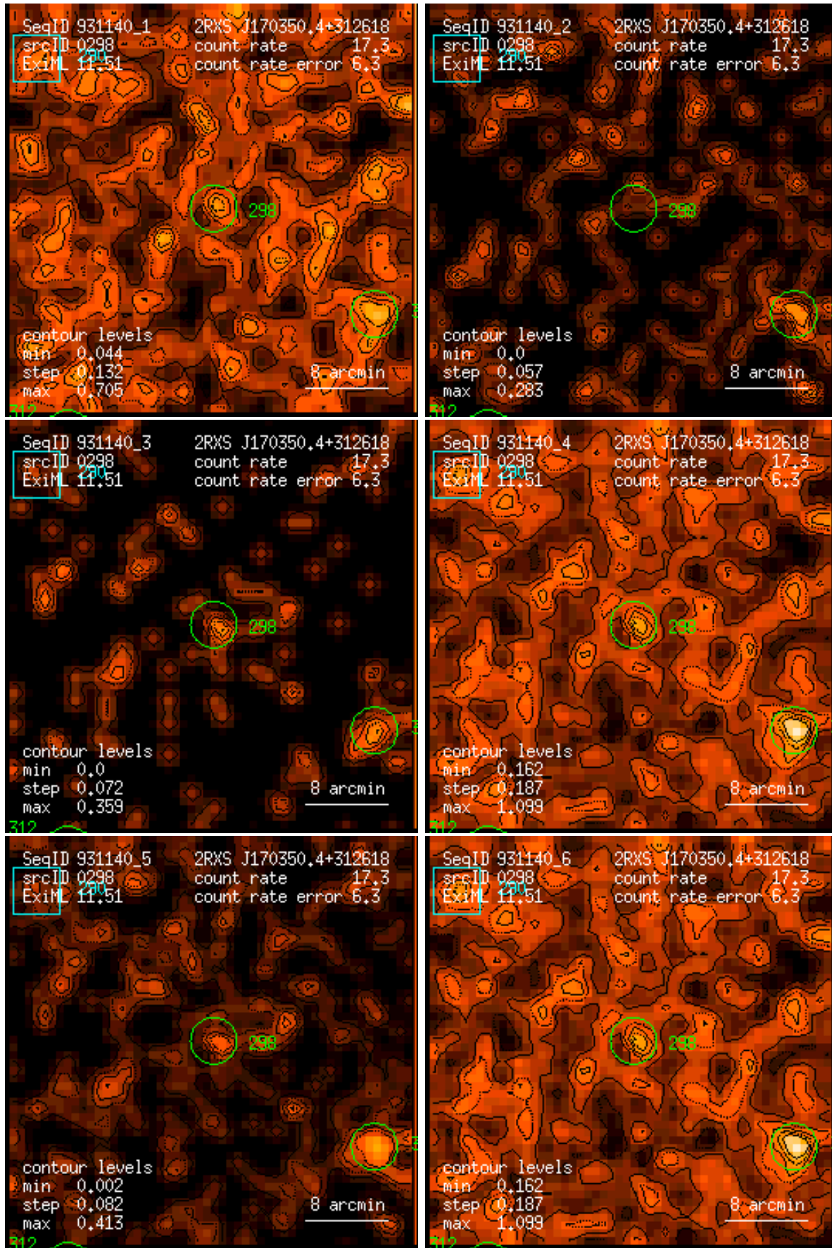
Figure 298: RASS 931140: detection 0298: band rate images, Gaussian filter: (1) PSPC channels 11 – 41, (2) 52 – 90, (3) 91 – 201, (4) 11 – 235, (5) 52 – 201, (6) 11 – 201. Broad band rates in counts/ks. Band rate contour levels in counts/ks/arcmin 2 .
