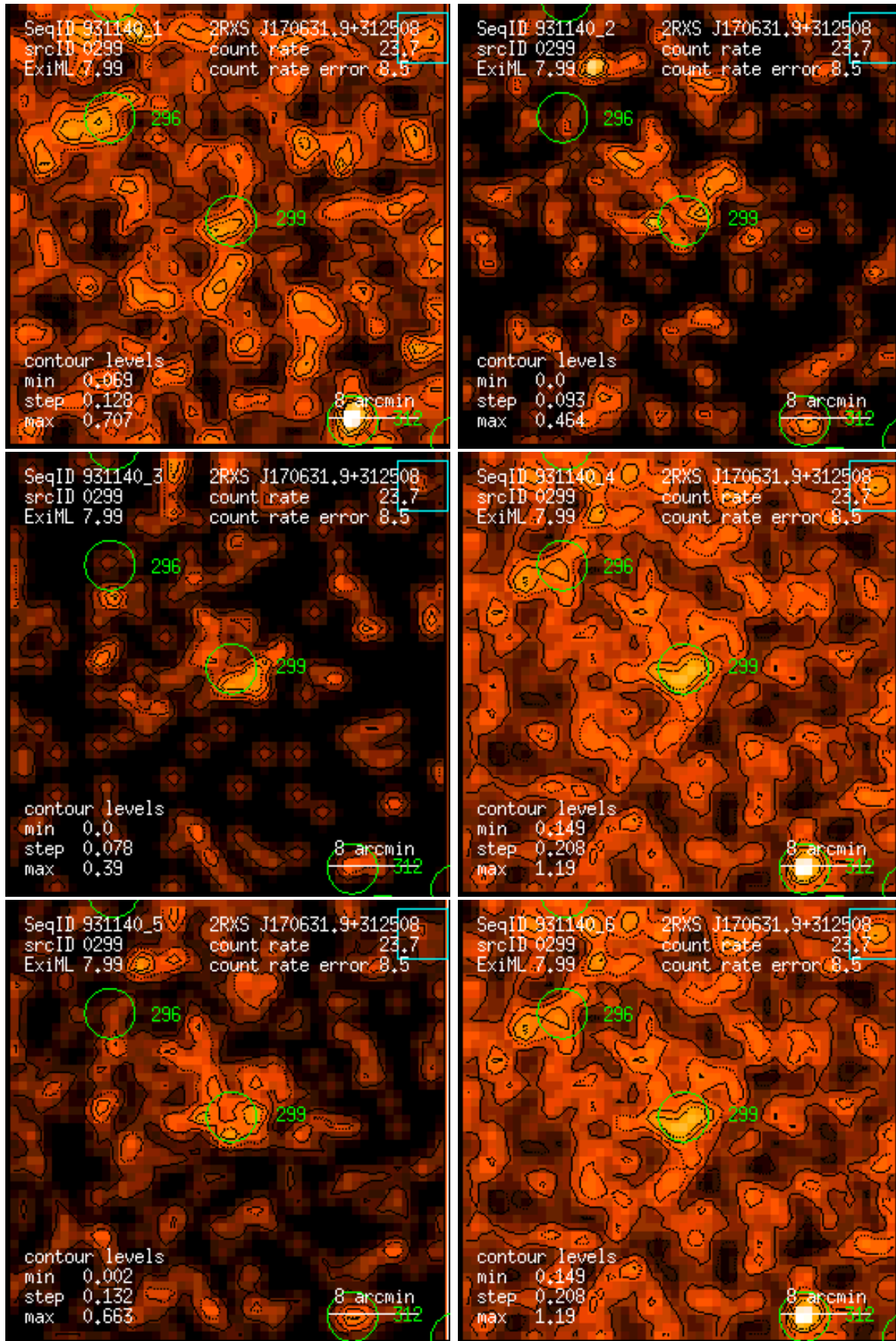
Figure 299: RASS 931140: detection 0299: band rate images, Gaussian filter: (1) PSPC channels 11 – 41, (2) 52 – 90, (3) 91 – 201, (4) 11 – 235, (5) 52 – 201, (6) 11 – 201. Broad band rates in counts/ks. Band rate contour levels in counts/ks/arcmin 2 .
