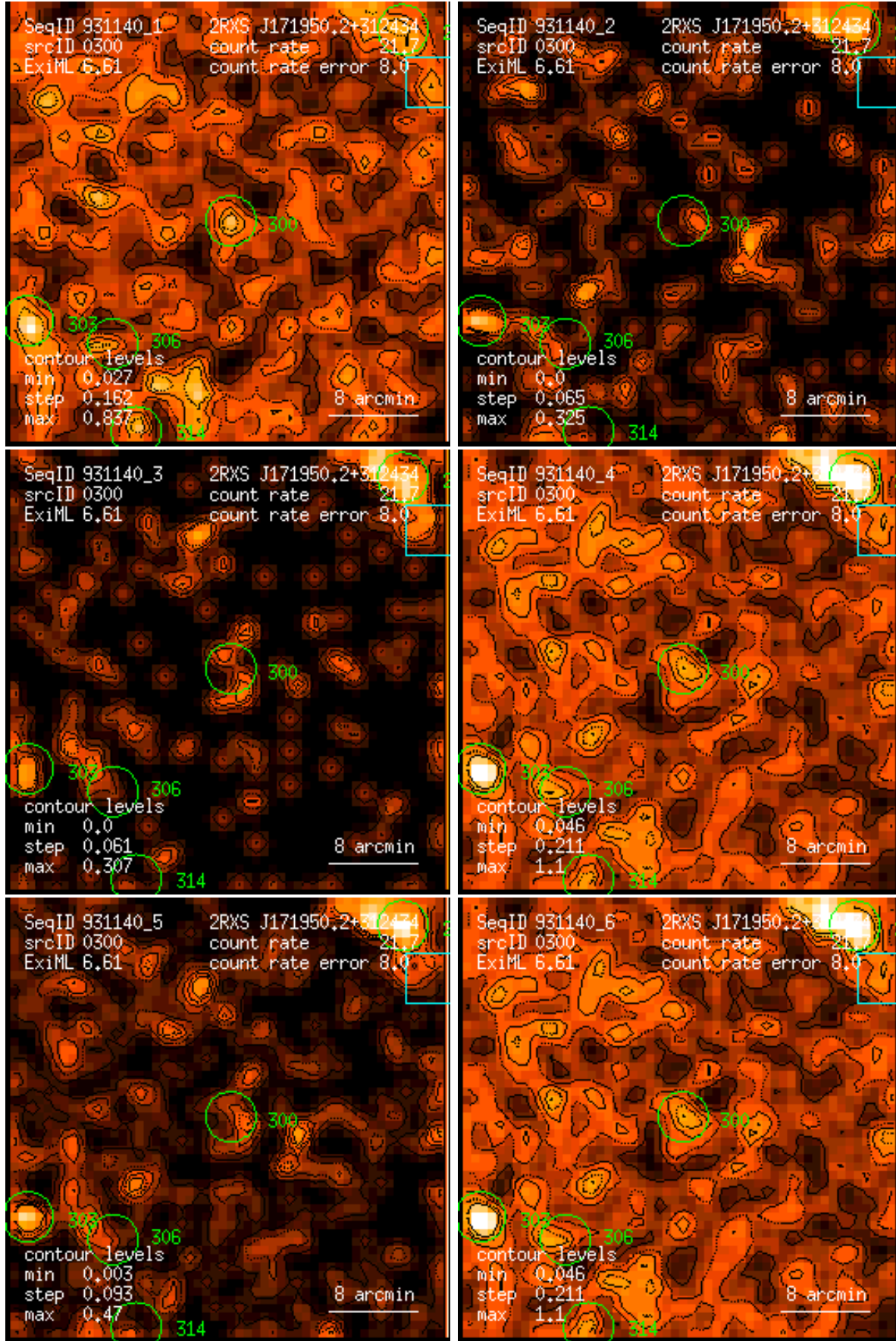
Figure 300: RASS 931140: detection 0300: band rate images, Gaussian filter: (1) PSPC channels 11 – 41, (2) 52 – 90, (3) 91 – 201, (4) 11 – 235, (5) 52 – 201, (6) 11 – 201. Broad band rates in counts/ks. Band rate contour levels in counts/ks/arcmin 2 .
