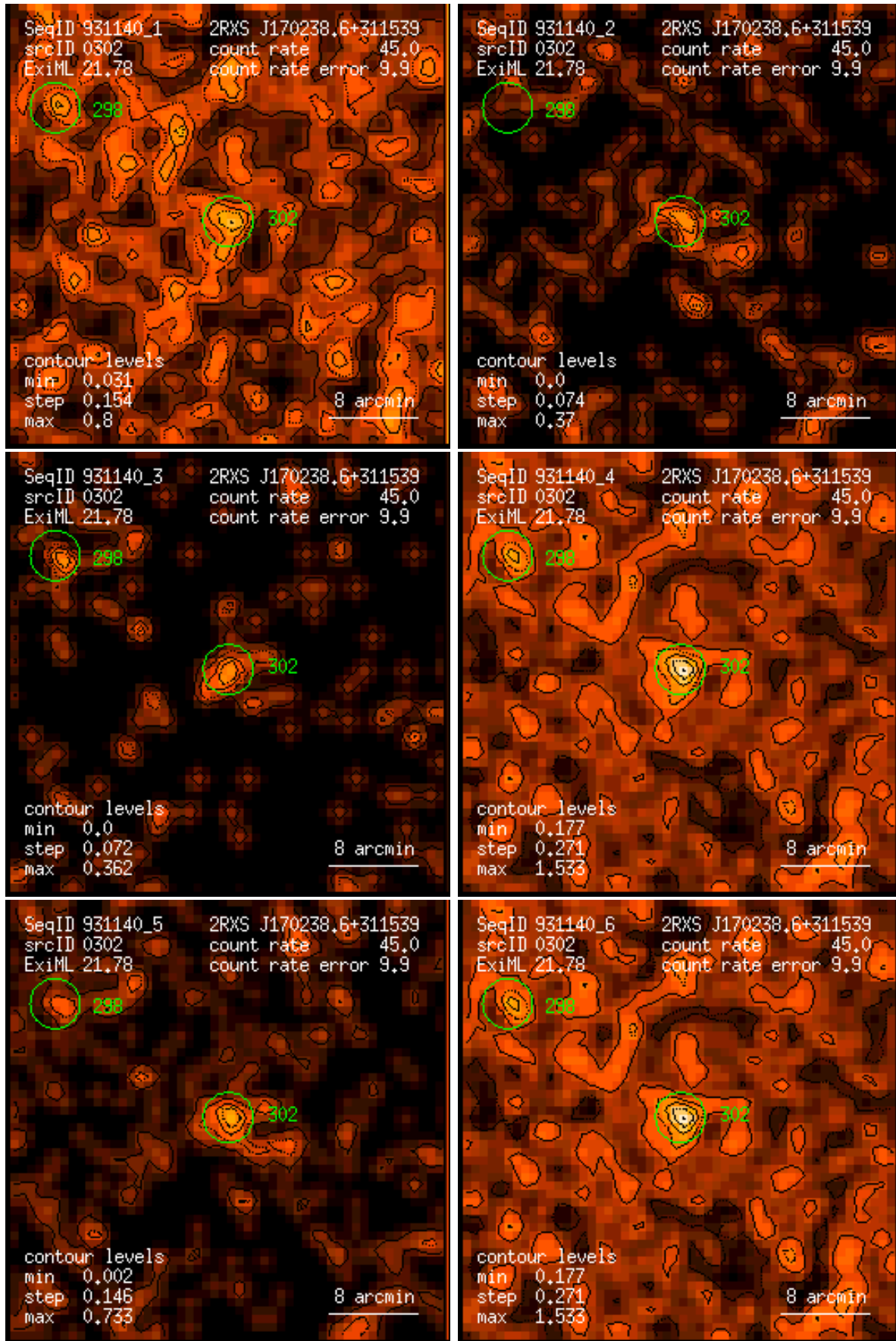
Figure 302: RASS 931140: detection 0302: band rate images, Gaussian filter: (1) PSPC channels 11 – 41, (2) 52 – 90, (3) 91 – 201, (4) 11 – 235, (5) 52 – 201, (6) 11 – 201. Broad band rates in counts/ks. Band rate contour levels in counts/ks/arcmin 2 .
