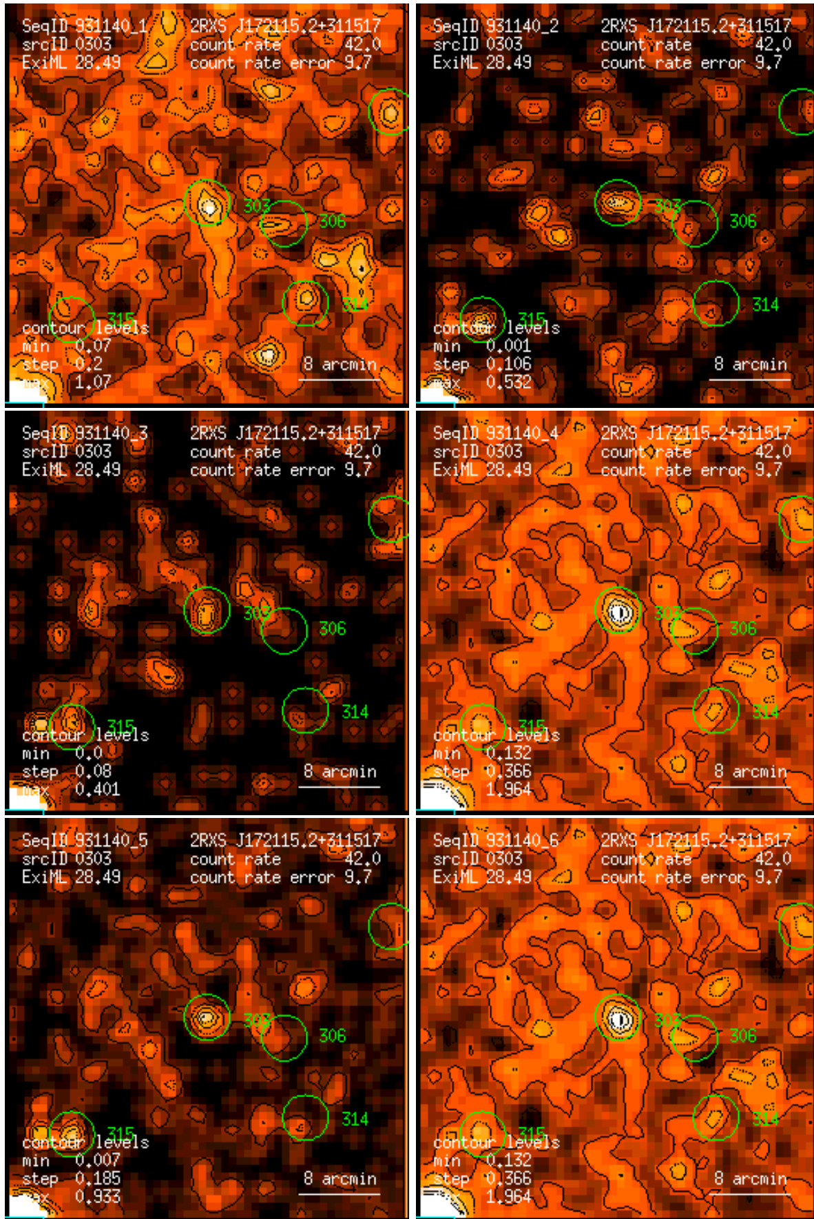
Figure 303: RASS 931140: detection 0303: band rate images, Gaussian filter: (1) PSPC channels 11 – 41, (2) 52 – 90, (3) 91 – 201, (4) 11 – 235, (5) 52 – 201, (6) 11 – 201. Broad band rates in counts/ks. Band rate contour levels in counts/ks/arcmin 2 .
