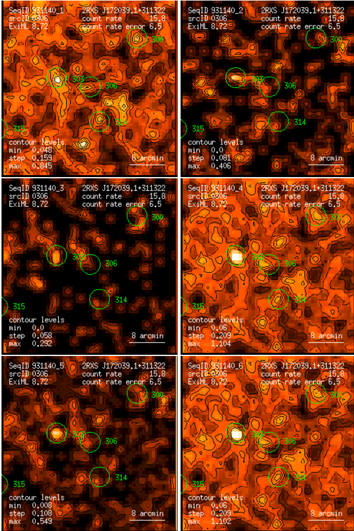
Figure 306: RASS 931140: detection 0306: band rate images, Gaussian filter: (1) PSPC channels 11 – 41, (2) 52 – 90, (3) 91 – 201, (4) 11 – 235, (5) 52 – 201, (6) 11 – 201. Broad band rates in counts/ks. Band rate contour levels in counts/ks/arcmin 2 .
