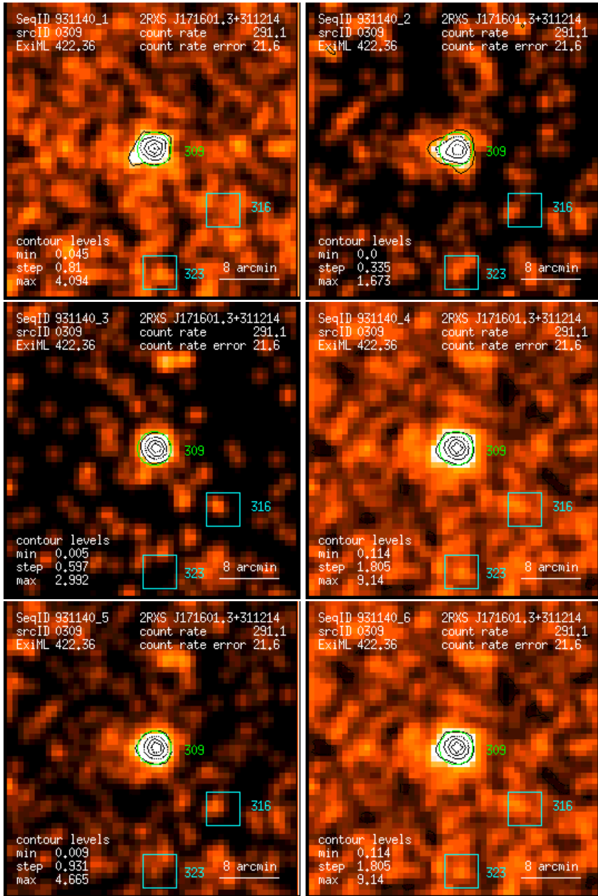
Figure 309: RASS 931140: detection 0309: band rate images, Gaussian filter: (1) PSPC channels 11 – 41, (2) 52 – 90, (3) 91 – 201, (4) 11 – 235, (5) 52 – 201, (6) 11 – 201. Broad band rates in counts/ks. Band rate contour levels in counts/ks/arcmin 2 .
