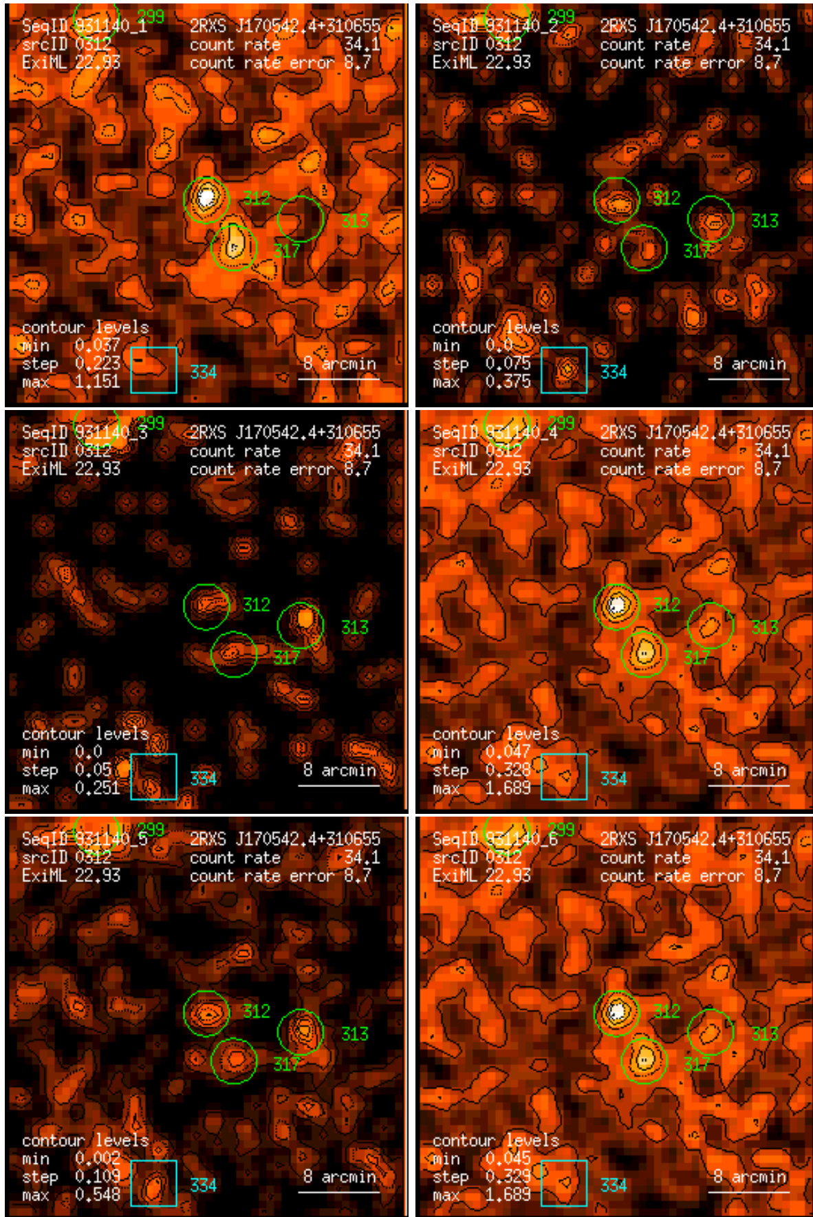
Figure 312: RASS 931140: detection 0312: band rate images, Gaussian filter: (1) PSPC channels 11 – 41, (2) 52 – 90, (3) 91 – 201, (4) 11 – 235, (5) 52 – 201, (6) 11 – 201. Broad band rates in counts/ks. Band rate contour levels in counts/ks/arcmin 2 .
