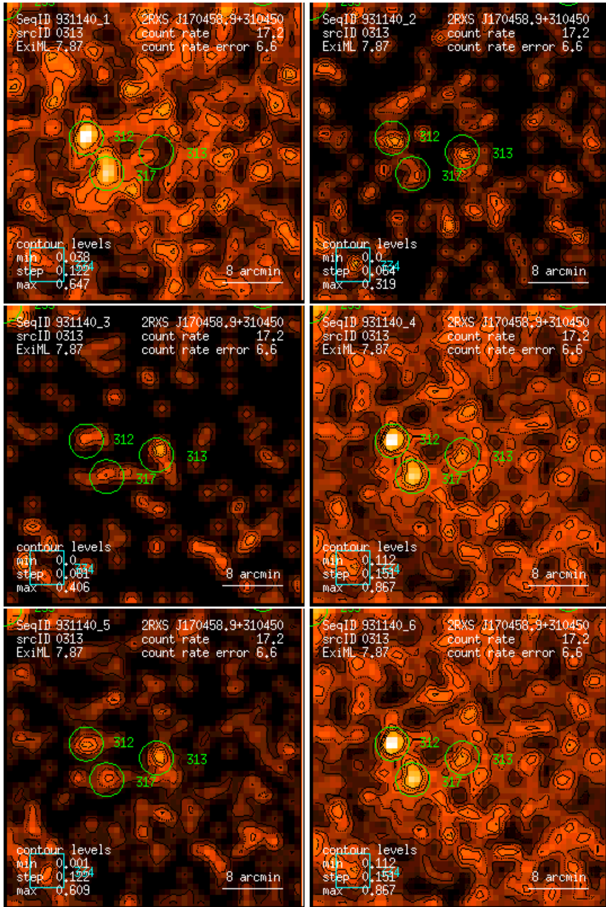
Figure 313: RASS 931140: detection 0313: band rate images, Gaussian filter: (1) PSPC channels 11 – 41, (2) 52 – 90, (3) 91 – 201, (4) 11 – 235, (5) 52 – 201, (6) 11 – 201. Broad band rates in counts/ks. Band rate contour levels in counts/ks/arcmin 2 .
