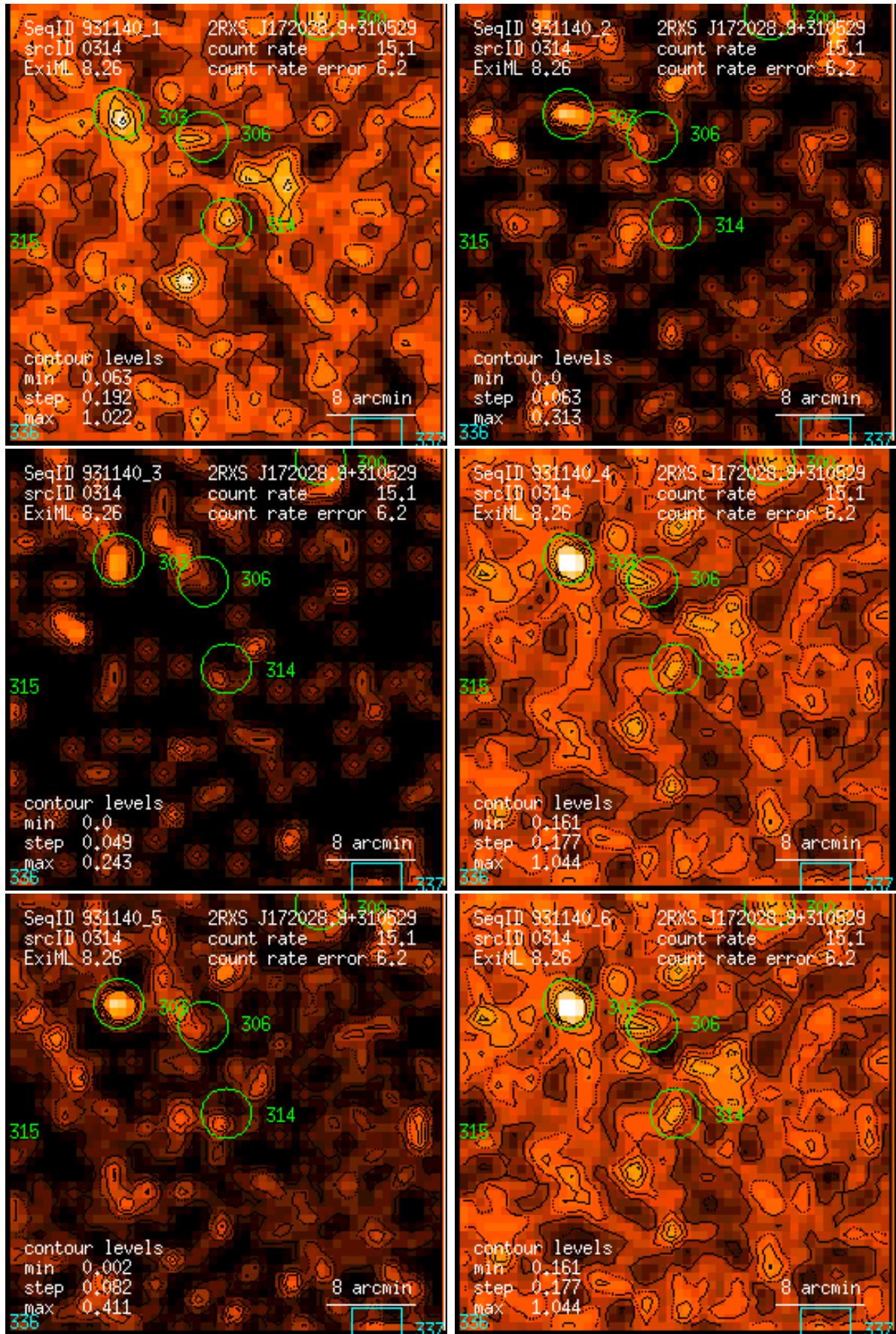
Figure 314: RASS 931140: detection 0314: band rate images, Gaussian filter: (1) PSPC channels 11 – 41, (2) 52 – 90, (3) 91 – 201, (4) 11 – 235, (5) 52 – 201, (6) 11 – 201. Broad band rates in counts/ks. Band rate contour levels in counts/ks/arcmin 2 .
