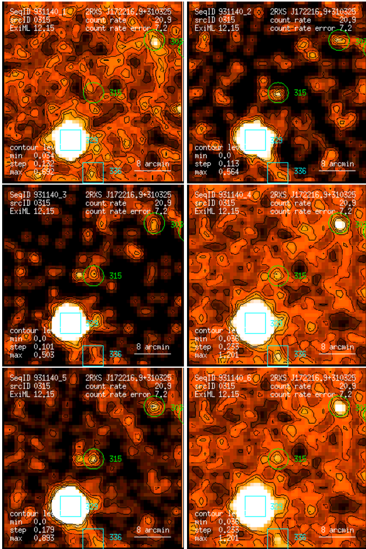
Figure 315: RASS 931140: detection 0315: band rate images, Gaussian filter: (1) PSPC channels 11 – 41, (2) 52 – 90, (3) 91 – 201, (4) 11 – 235, (5) 52 – 201, (6) 11 – 201. Broad band rates in counts/ks. Band rate contour levels in counts/ks/arcmin 2 .
