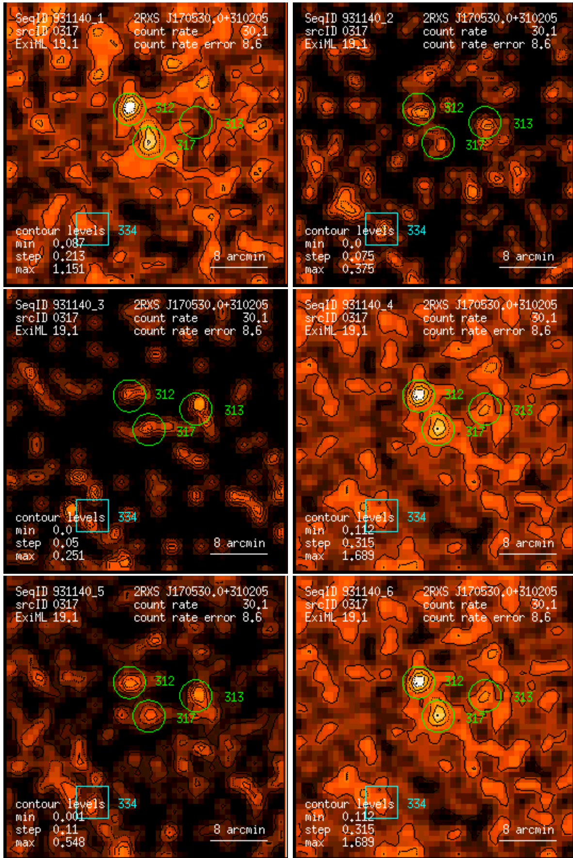
Figure 317: RASS 931140: detection 0317: band rate images, Gaussian filter: (1) PSPC channels 11 – 41, (2) 52 – 90, (3) 91 – 201, (4) 11 – 235, (5) 52 – 201, (6) 11 – 201. Broad band rates in counts/ks. Band rate contour levels in counts/ks/arcmin 2 .
