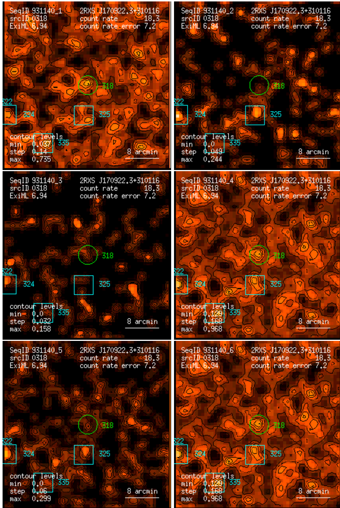
Figure 318: RASS 931140: detection 0318: band rate images, Gaussian filter: (1) PSPC channels 11 – 41, (2) 52 – 90, (3) 91 – 201, (4) 11 – 235, (5) 52 – 201, (6) 11 – 201. Broad band rates in counts/ks. Band rate contour levels in counts/ks/arcmin 2 .
