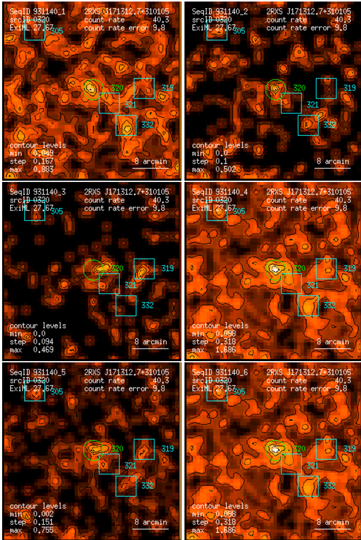
Figure 320: RASS 931140: detection 0320: band rate images, Gaussian filter: (1) PSPC channels 11 – 41, (2) 52 – 90, (3) 91 – 201, (4) 11 – 235, (5) 52 – 201, (6) 11 – 201. Broad band rates in counts/ks. Band rate contour levels in counts/ks/arcmin 2 .
