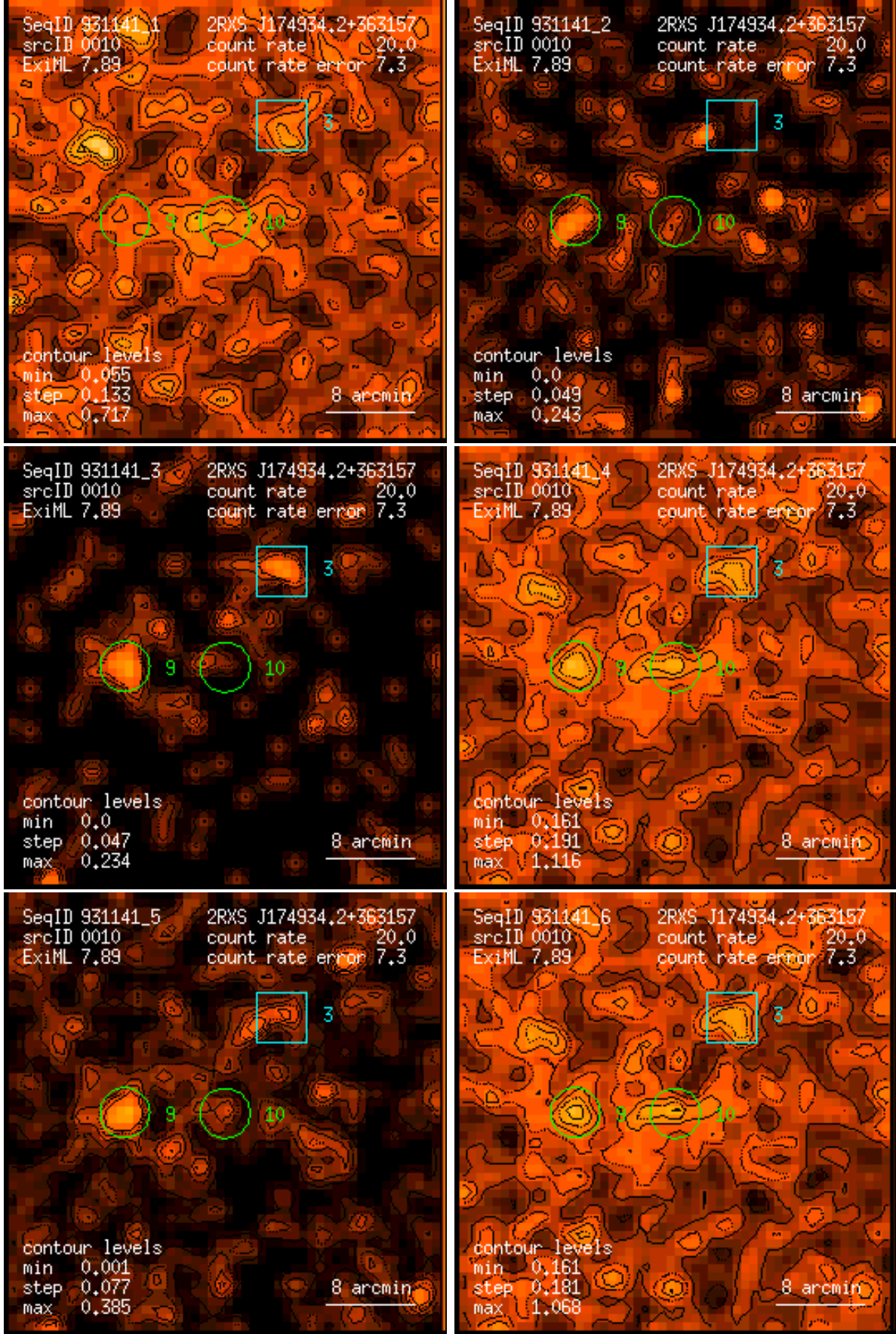
Figure 10: RASS 931141: detection 0010: band rate images, Gaussian filter: (1) PSPC channels 11 – 41, (2) 52 – 90, (3) 91 – 201, (4) 11 – 235, (5) 52 – 201, (6) 11 – 201. Broad band rates in counts/ks. Band rate contour levels in counts/ks/arcmin 2 .
