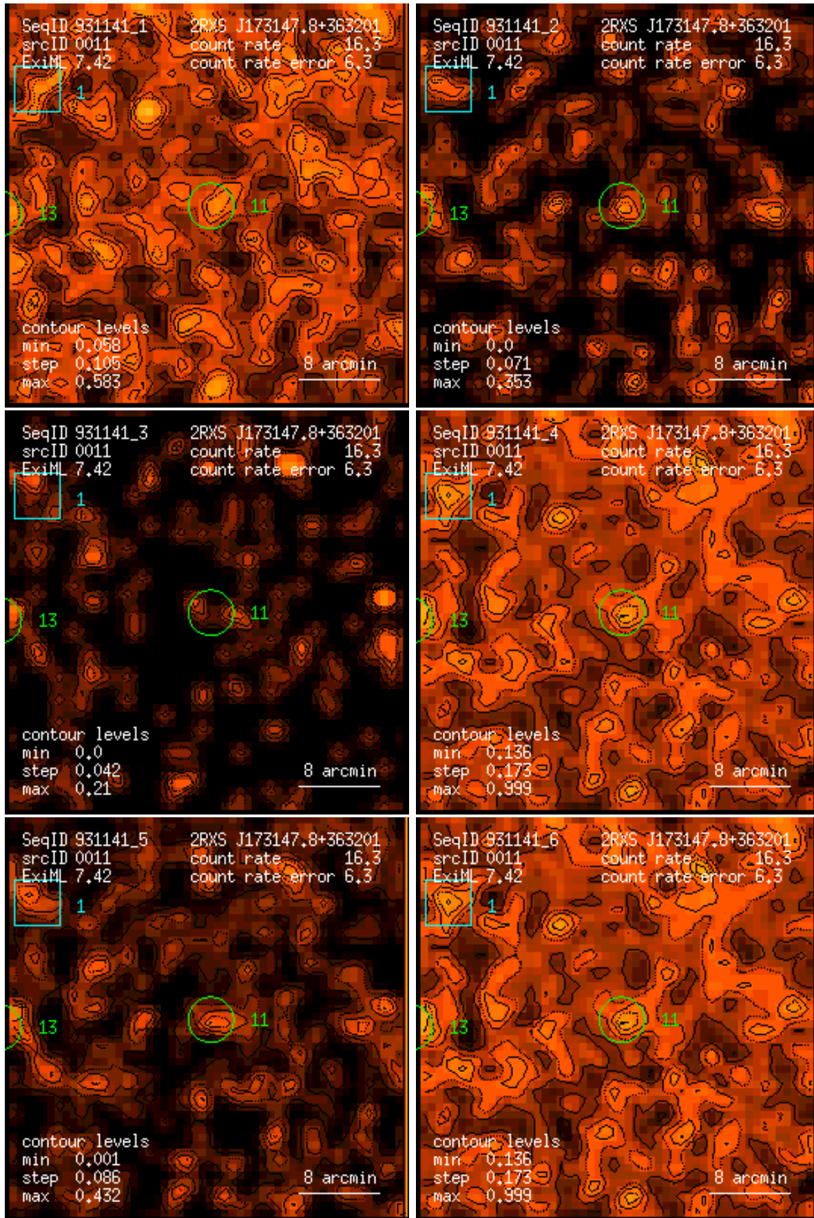
Figure 11: RASS 931141: detection 0011: band rate images, Gaussian filter: (1) PSPC channels 11 – 41, (2) 52 – 90, (3) 91 – 201, (4) 11 – 235, (5) 52 – 201, (6) 11 – 201. Broad band rates in counts/ks. Band rate contour levels in counts/ks/arcmin 2 .
