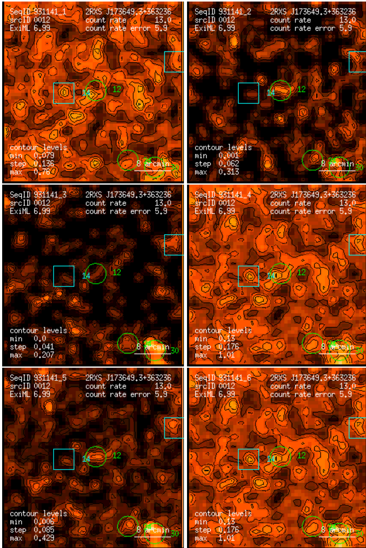
Figure 12: RASS 931141: detection 0012: band rate images, Gaussian filter: (1) PSPC channels 11 – 41, (2) 52 – 90, (3) 91 – 201, (4) 11 – 235, (5) 52 – 201, (6) 11 – 201. Broad band rates in counts/ks. Band rate contour levels in counts/ks/arcmin 2 .
