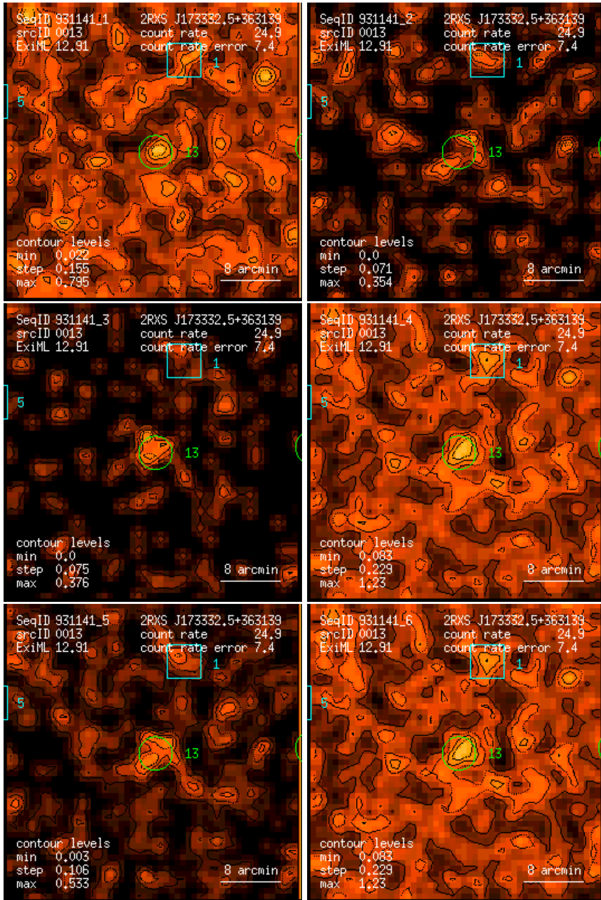
Figure 13: RASS 931141: detection 0013: band rate images, Gaussian filter: (1) PSPC channels 11 – 41, (2) 52 – 90, (3) 91 – 201, (4) 11 – 235, (5) 52 – 201, (6) 11 – 201. Broad band rates in counts/ks. Band rate contour levels in counts/ks/arcmin 2 .
