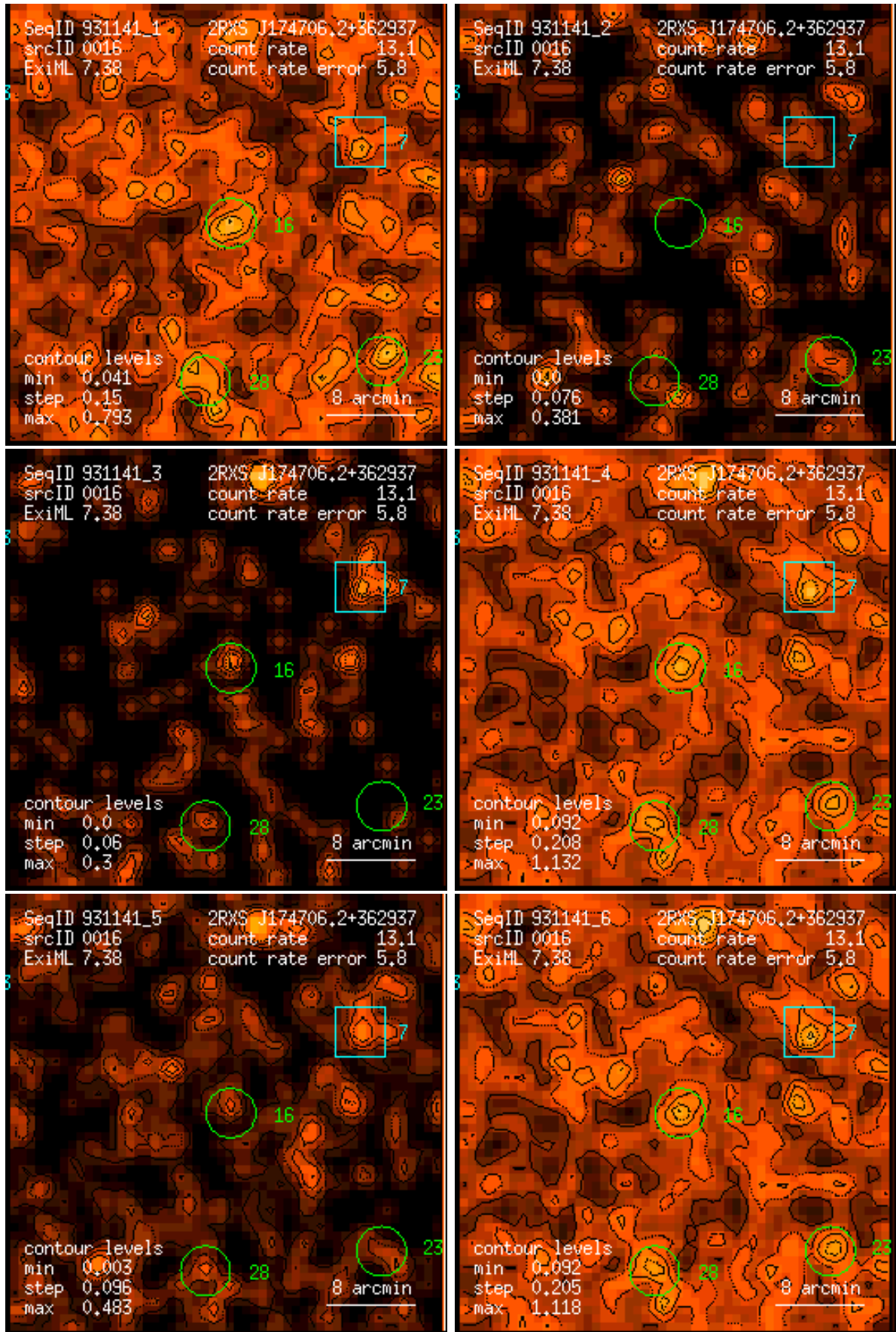
Figure 16: RASS 931141: detection 0016: band rate images, Gaussian filter: (1) PSPC channels 11 – 41, (2) 52 – 90, (3) 91 – 201, (4) 11 – 235, (5) 52 – 201, (6) 11 – 201. Broad band rates in counts/ks. Band rate contour levels in counts/ks/arcmin 2 .
