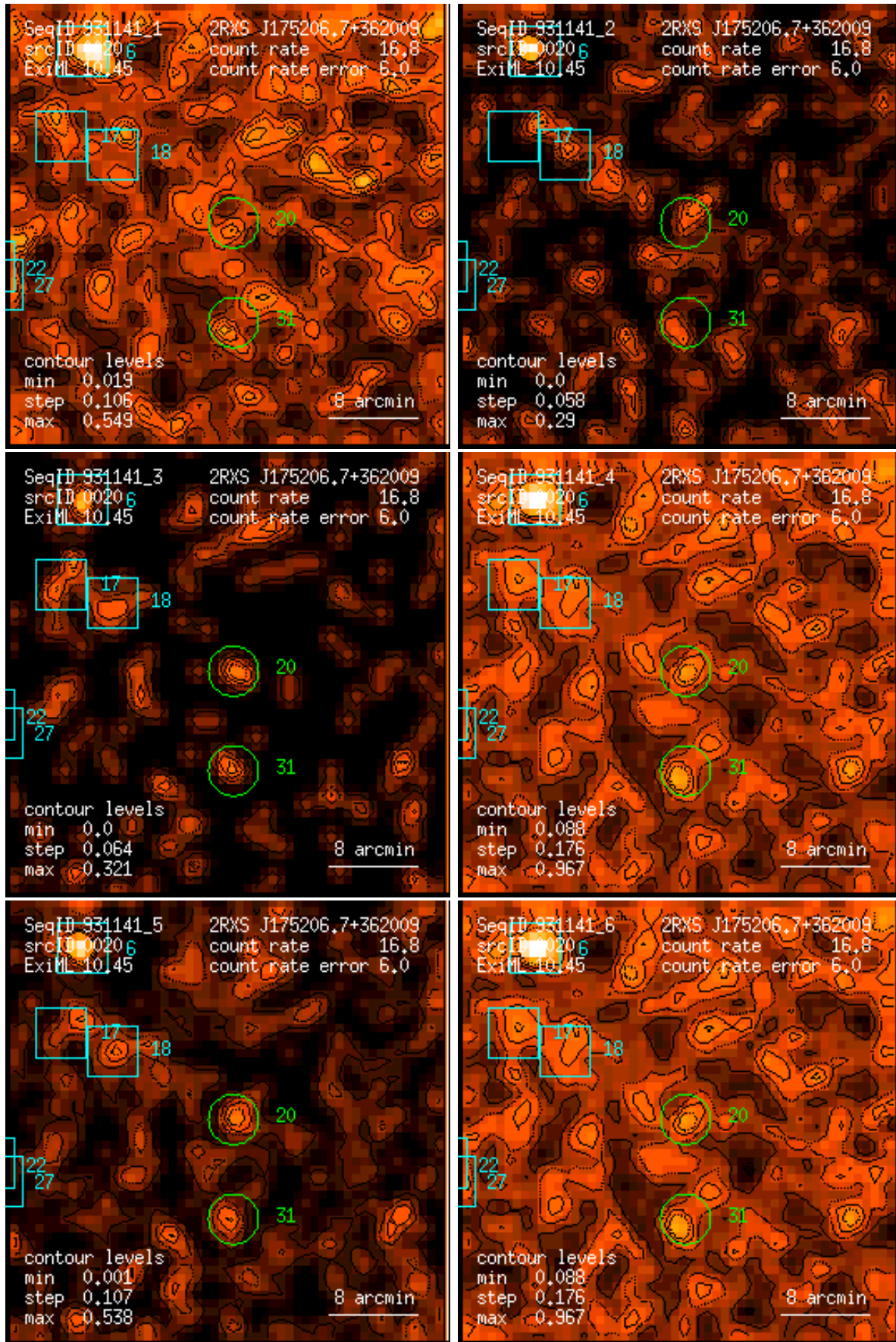
Figure 20: RASS 931141: detection 0020: band rate images, Gaussian filter: (1) PSPC channels 11 – 41, (2) 52 – 90, (3) 91 – 201, (4) 11 – 235, (5) 52 – 201, (6) 11 – 201. Broad band rates in counts/ks. Band rate contour levels in counts/ks/arcmin 2 .
