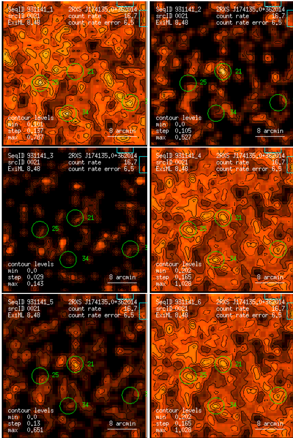
Figure 21: RASS 931141: detection 0021: band rate images, Gaussian filter: (1) PSPC channels 11 – 41, (2) 52 – 90, (3) 91 – 201, (4) 11 – 235, (5) 52 – 201, (6) 11 – 201. Broad band rates in counts/ks. Band rate contour levels in counts/ks/arcmin 2 .
