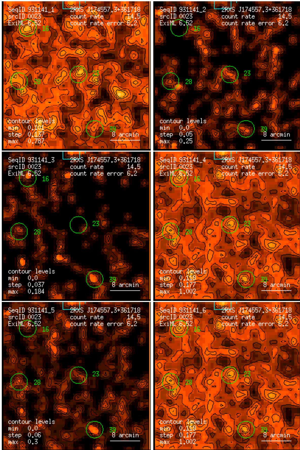
Figure 23: RASS 931141: detection 0023: band rate images, Gaussian filter: (1) PSPC channels 11 – 41, (2) 52 – 90, (3) 91 – 201, (4) 11 – 235, (5) 52 – 201, (6) 11 – 201. Broad band rates in counts/ks. Band rate contour levels in counts/ks/arcmin 2 .
