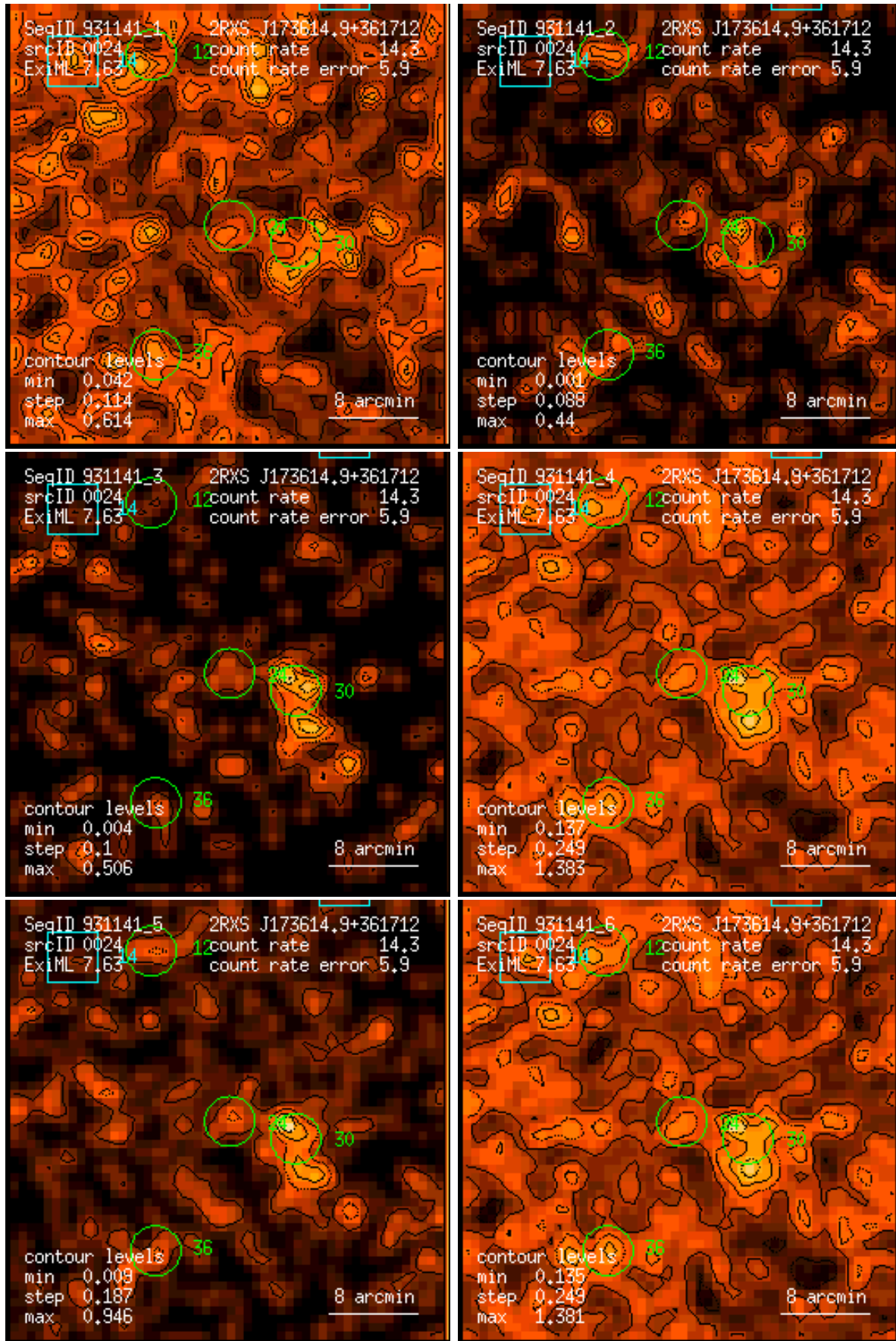
Figure 24: RASS 931141: detection 0024: band rate images, Gaussian filter: (1) PSPC channels 11 – 41, (2) 52 – 90, (3) 91 – 201, (4) 11 – 235, (5) 52 – 201, (6) 11 – 201. Broad band rates in counts/ks. Band rate contour levels in counts/ks/arcmin 2 .
