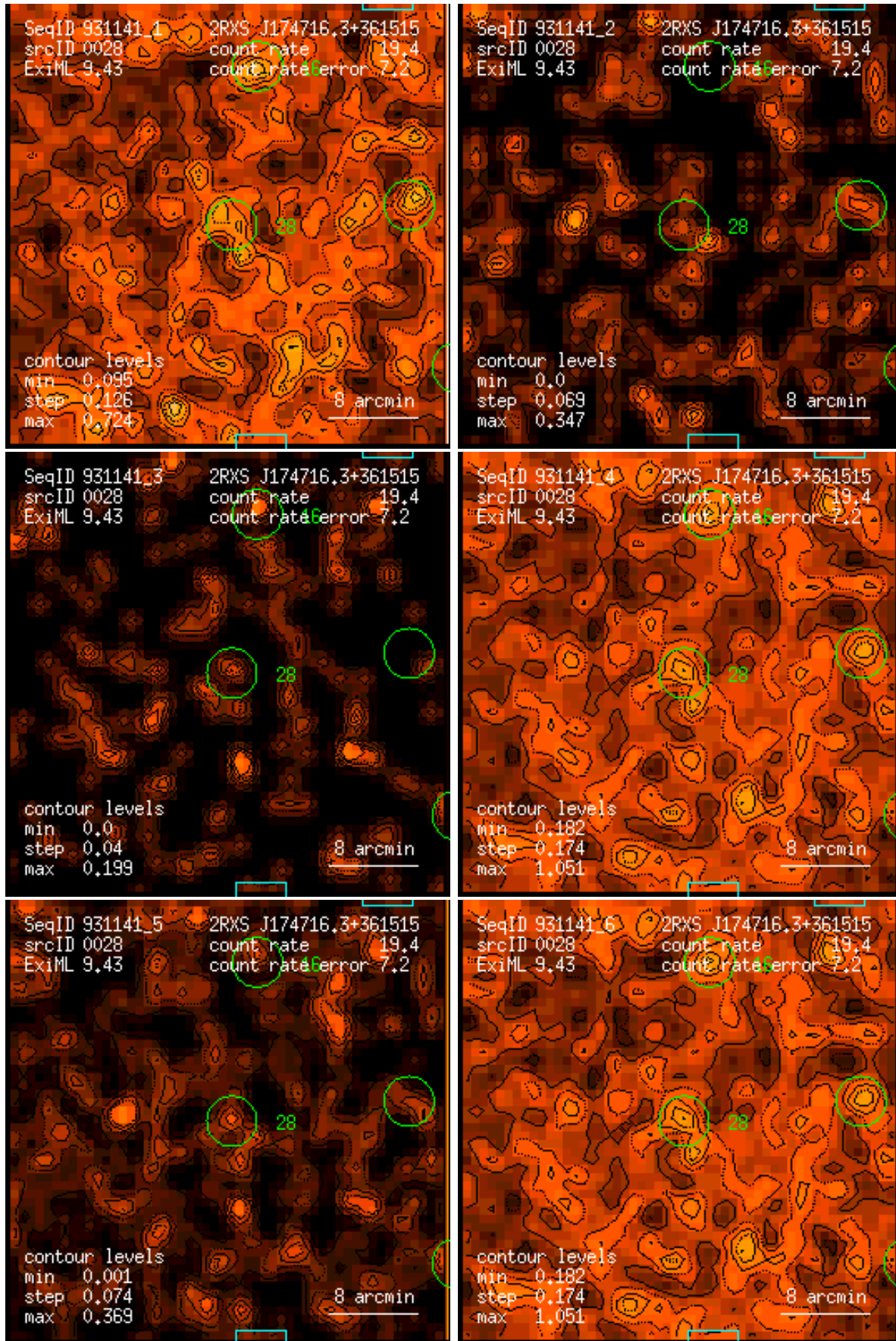
Figure 28: RASS 931141: detection 0028: band rate images, Gaussian filter: (1) PSPC channels 11 – 41, (2) 52 – 90, (3) 91 – 201, (4) 11 – 235, (5) 52 – 201, (6) 11 – 201. Broad band rates in counts/ks. Band rate contour levels in counts/ks/arcmin 2 .
