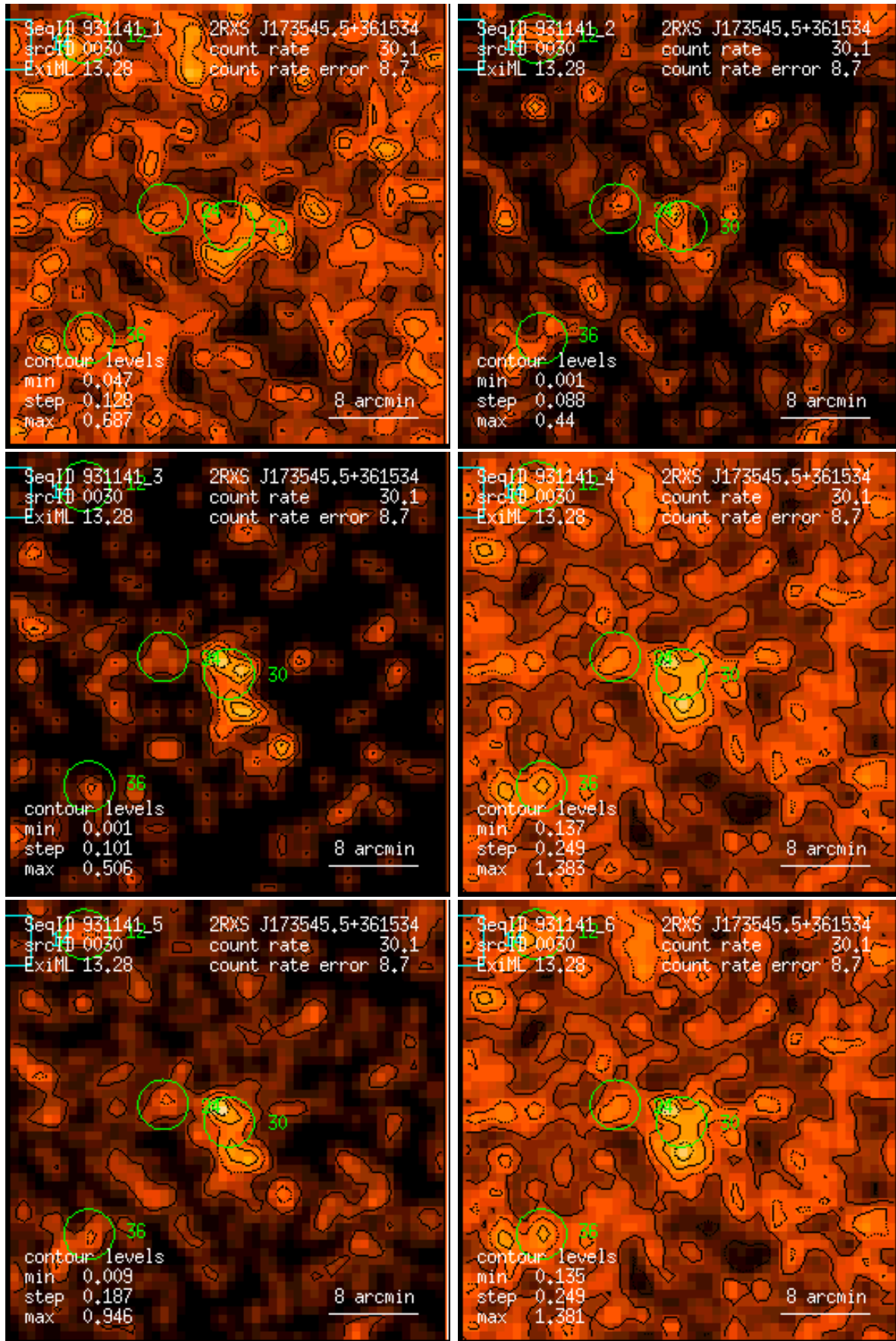
Figure 30: RASS 931141: detection 0030: band rate images, Gaussian filter: (1) PSPC channels 11 – 41, (2) 52 – 90, (3) 91 – 201, (4) 11 – 235, (5) 52 – 201, (6) 11 – 201. Broad band rates in counts/ks. Band rate contour levels in counts/ks/arcmin 2 .
