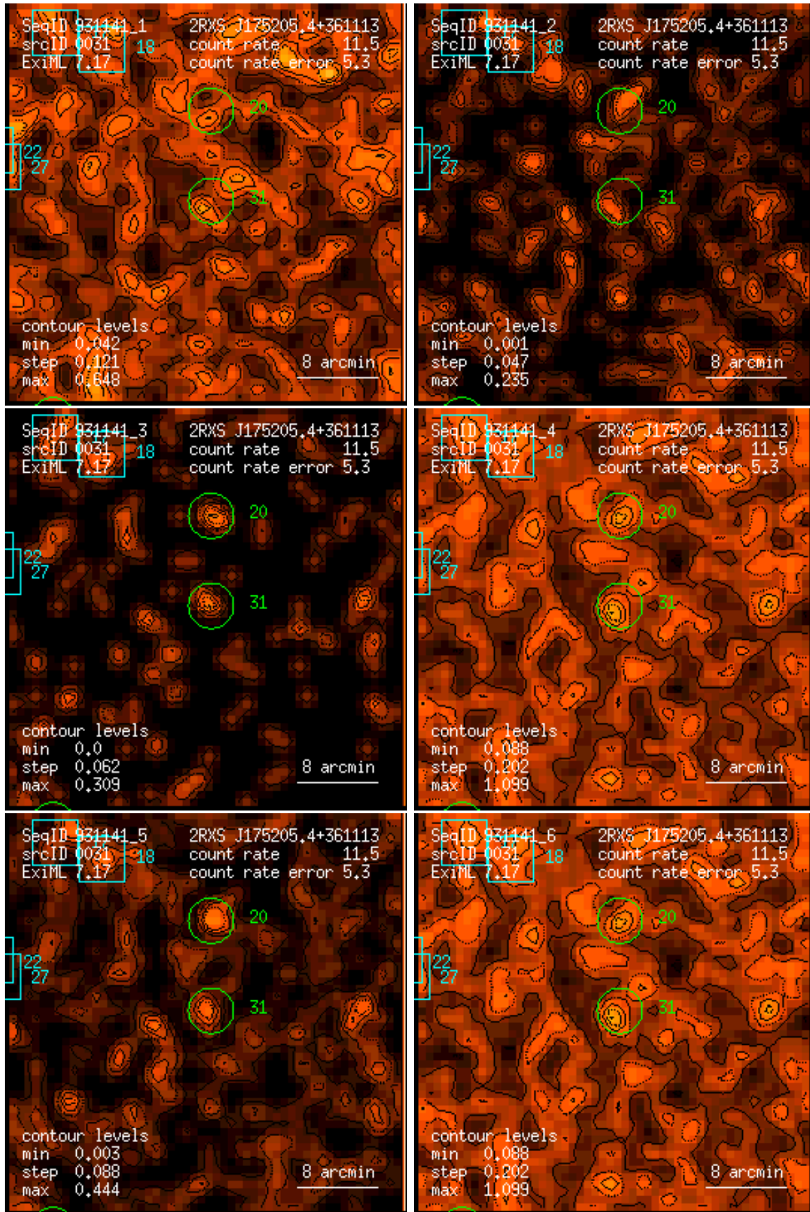
Figure 31: RASS 931141: detection 0031: band rate images, Gaussian filter: (1) PSPC channels 11 – 41, (2) 52 – 90, (3) 91 – 201, (4) 11 – 235, (5) 52 – 201, (6) 11 – 201. Broad band rates in counts/ks. Band rate contour levels in counts/ks/arcmin 2 .
