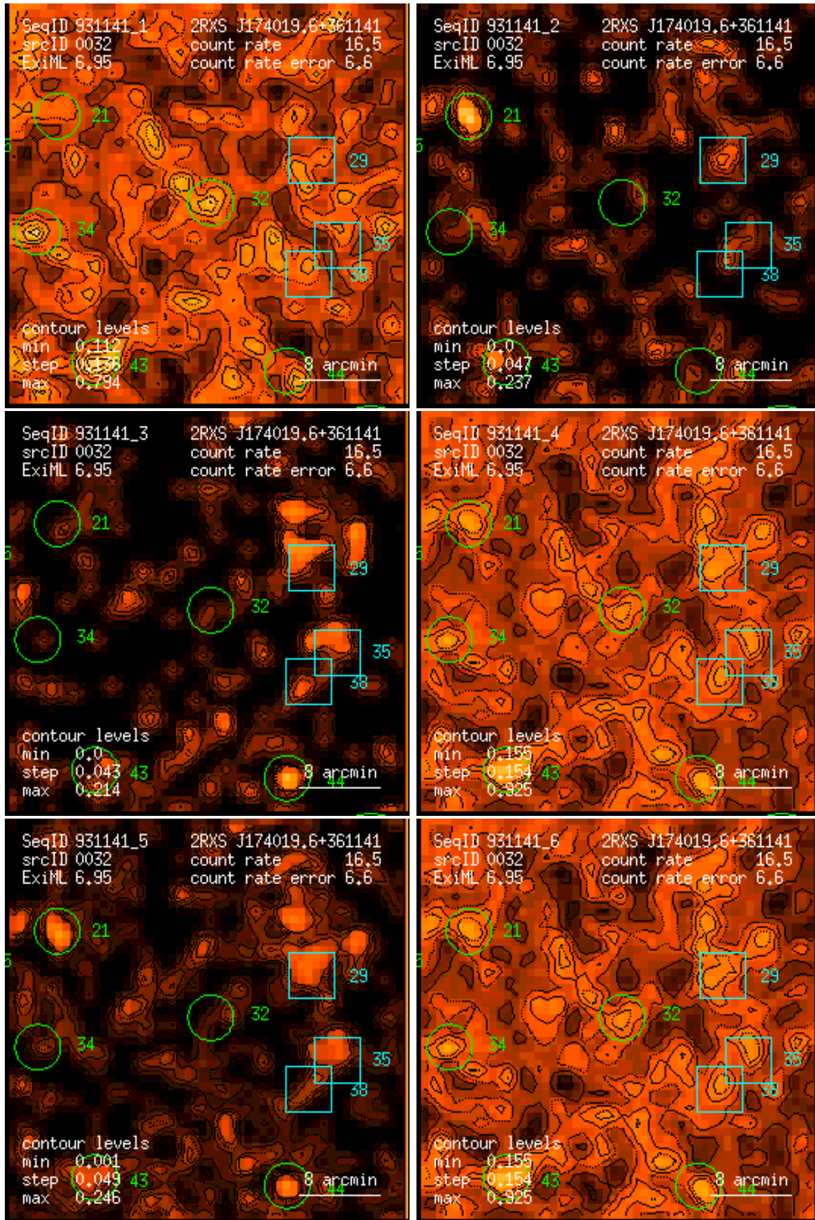
Figure 32: RASS 931141: detection 0032: band rate images, Gaussian filter: (1) PSPC channels 11 – 41, (2) 52 – 90, (3) 91 – 201, (4) 11 – 235, (5) 52 – 201, (6) 11 – 201. Broad band rates in counts/ks. Band rate contour levels in counts/ks/arcmin 2 .
