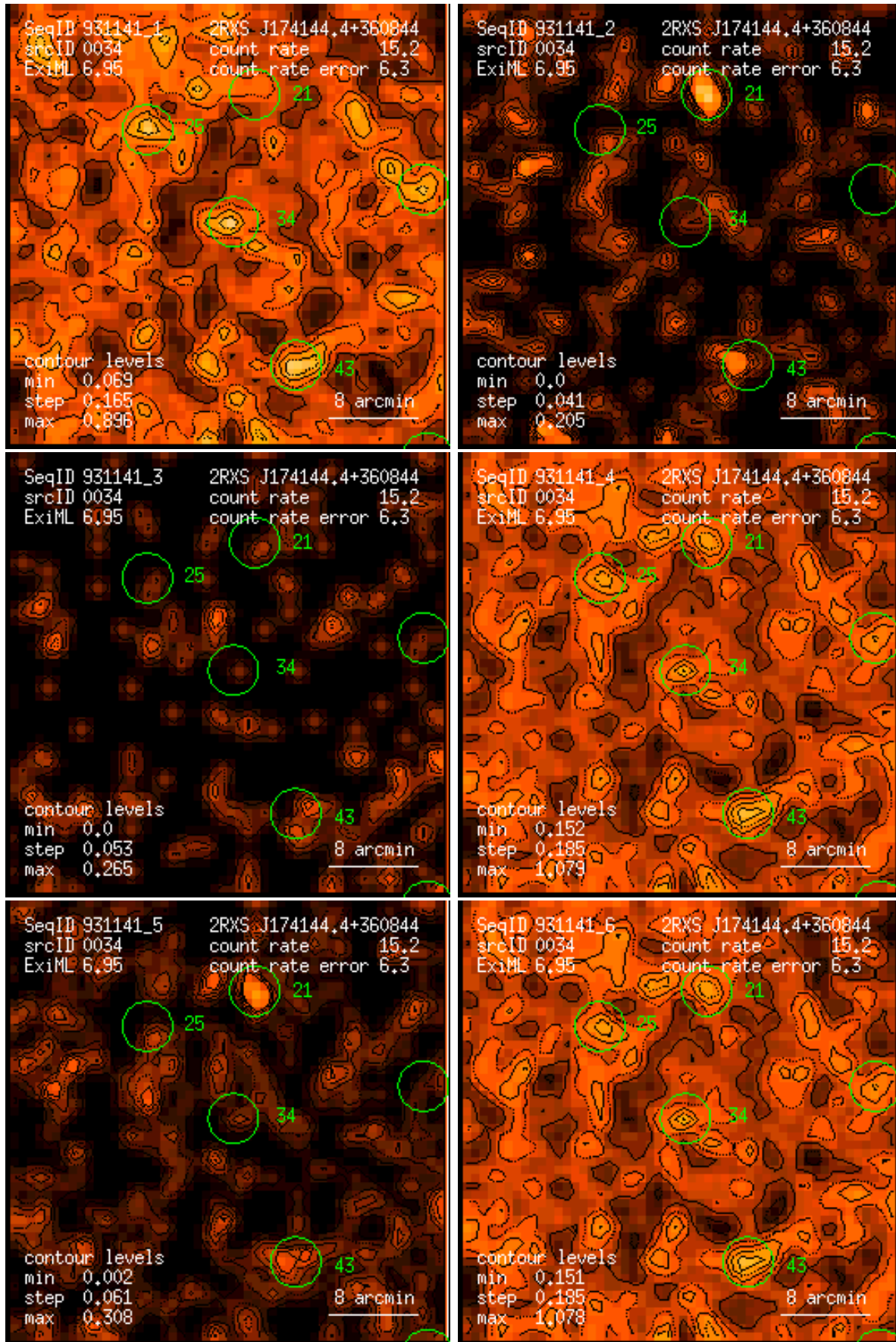
Figure 34: RASS 931141: detection 0034: band rate images, Gaussian filter: (1) PSPC channels 11 – 41, (2) 52 – 90, (3) 91 – 201, (4) 11 – 235, (5) 52 – 201, (6) 11 – 201. Broad band rates in counts/ks. Band rate contour levels in counts/ks/arcmin 2 .
