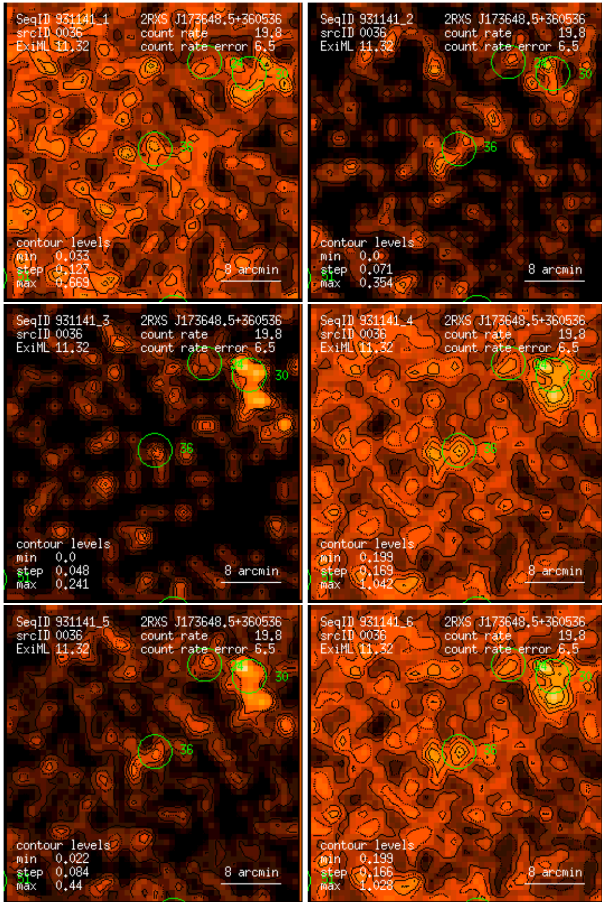
Figure 36: RASS 931141: detection 0036: band rate images, Gaussian filter: (1) PSPC channels 11 – 41, (2) 52 – 90, (3) 91 – 201, (4) 11 – 235, (5) 52 – 201, (6) 11 – 201. Broad band rates in counts/ks. Band rate contour levels in counts/ks/arcmin 2 .
