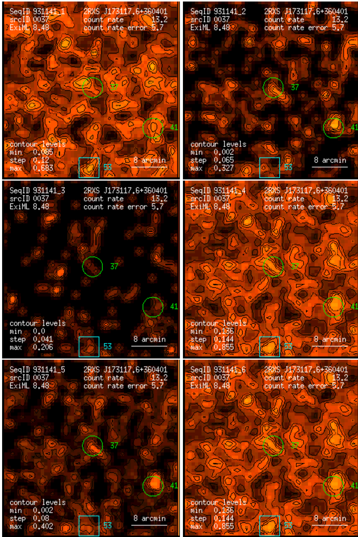
Figure 37: RASS 931141: detection 0037: band rate images, Gaussian filter: (1) PSPC channels 11 – 41, (2) 52 – 90, (3) 91 – 201, (4) 11 – 235, (5) 52 – 201, (6) 11 – 201. Broad band rates in counts/ks. Band rate contour levels in counts/ks/arcmin 2 .
