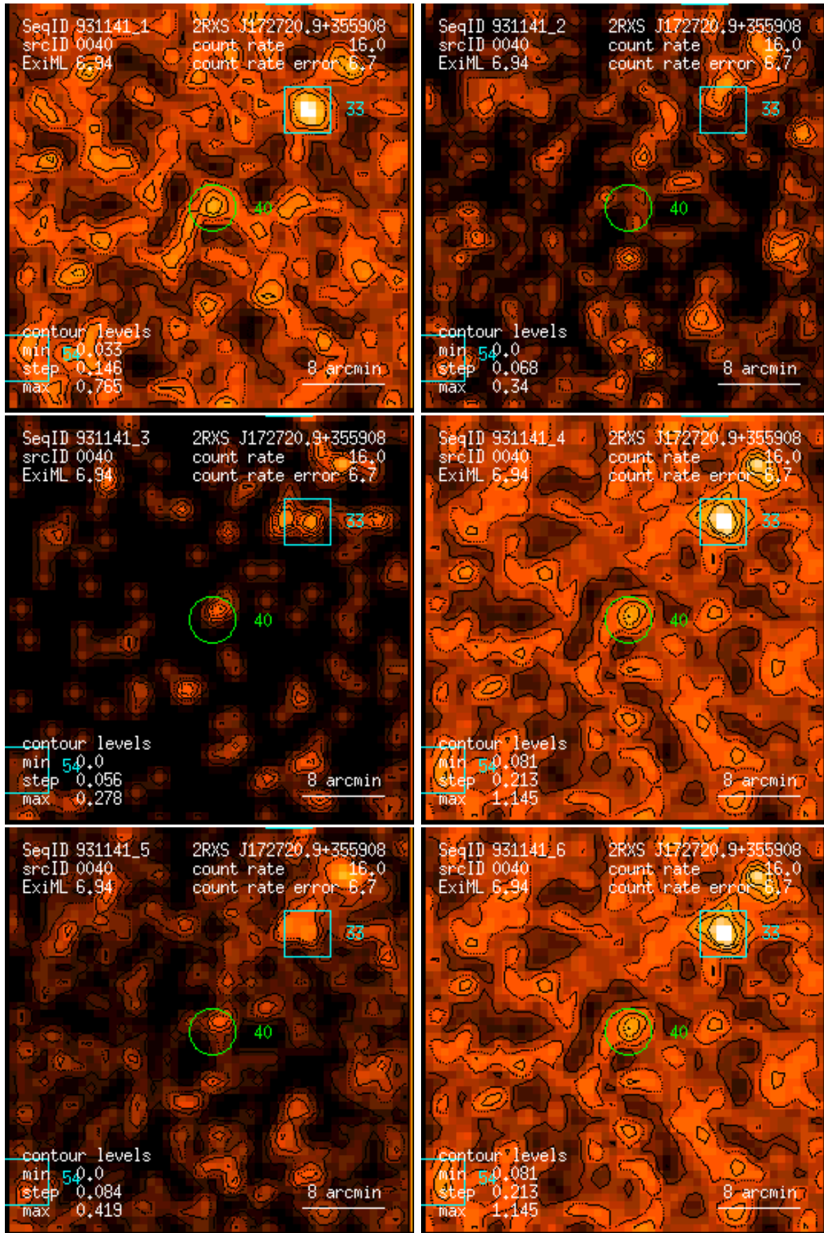
Figure 40: RASS 931141: detection 0040: band rate images, Gaussian filter: (1) PSPC channels 11 – 41, (2) 52 – 90, (3) 91 – 201, (4) 11 – 235, (5) 52 – 201, (6) 11 – 201. Broad band rates in counts/ks. Band rate contour levels in counts/ks/arcmin 2 .
