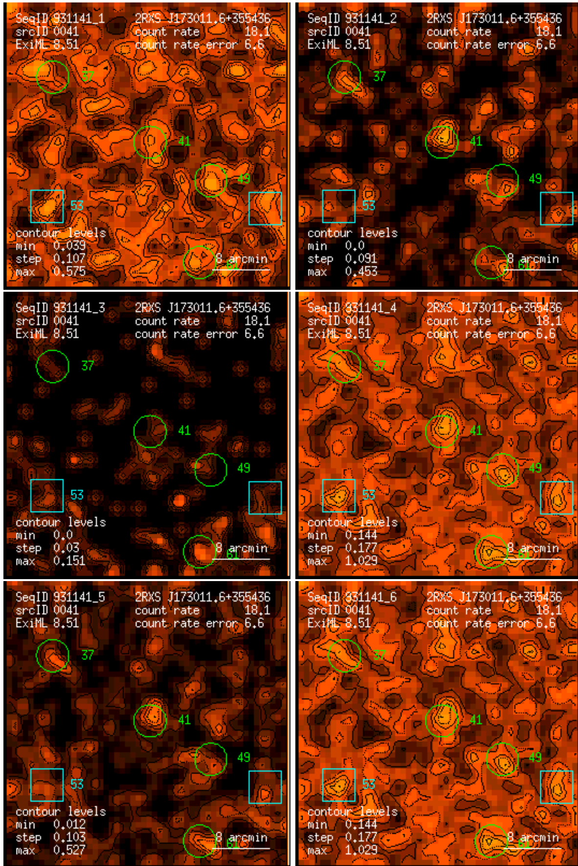
Figure 41: RASS 931141: detection 0041: band rate images, Gaussian filter: (1) PSPC channels 11 – 41, (2) 52 – 90, (3) 91 – 201, (4) 11 – 235, (5) 52 – 201, (6) 11 – 201. Broad band rates in counts/ks. Band rate contour levels in counts/ks/arcmin 2 .
