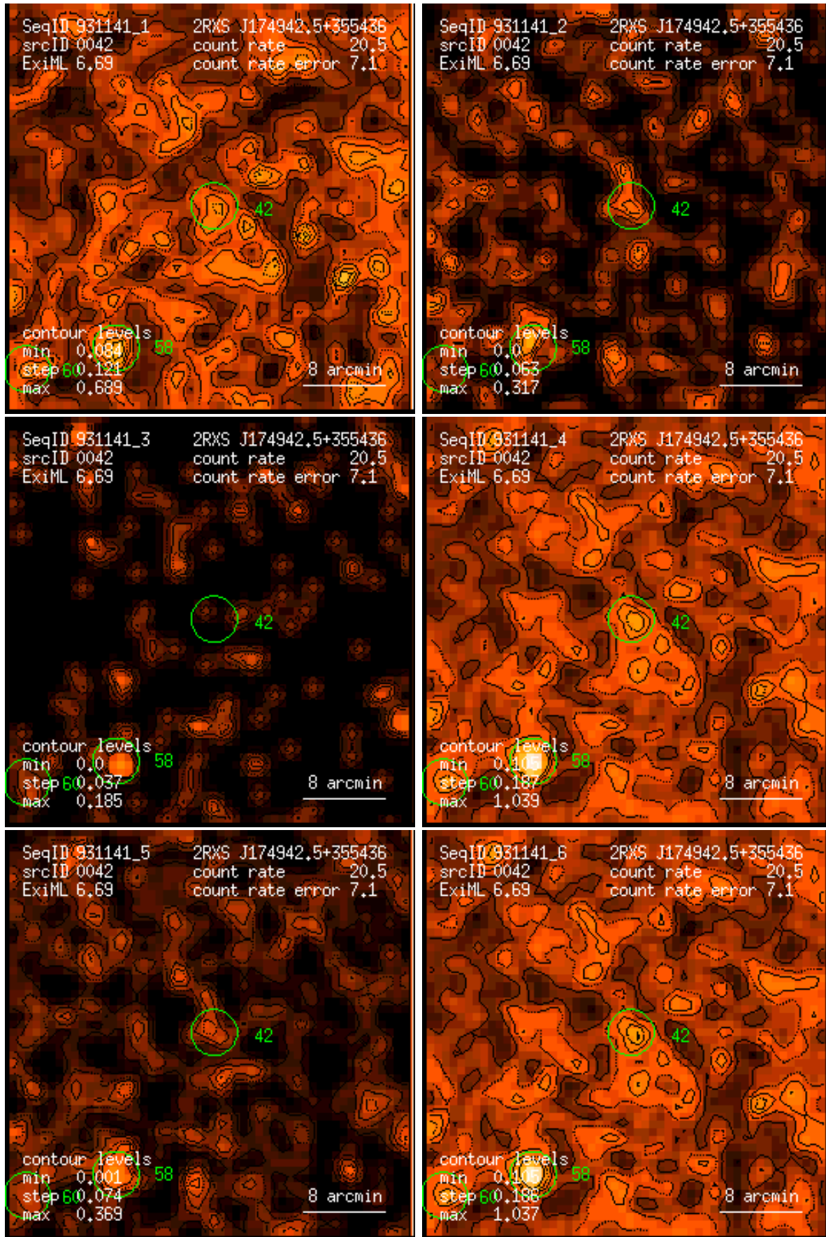
Figure 42: RASS 931141: detection 0042: band rate images, Gaussian filter: (1) PSPC channels 11 – 41, (2) 52 – 90, (3) 91 – 201, (4) 11 – 235, (5) 52 – 201, (6) 11 – 201. Broad band rates in counts/ks. Band rate contour levels in counts/ks/arcmin 2 .
