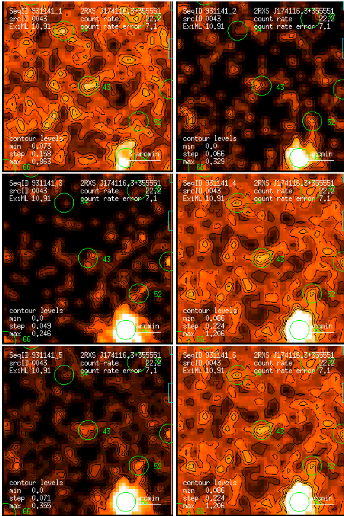
Figure 43: RASS 931141: detection 0043: band rate images, Gaussian filter: (1) PSPC channels 11 – 41, (2) 52 – 90, (3) 91 – 201, (4) 11 – 235, (5) 52 – 201, (6) 11 – 201. Broad band rates in counts/ks. Band rate contour levels in counts/ks/arcmin 2 .
