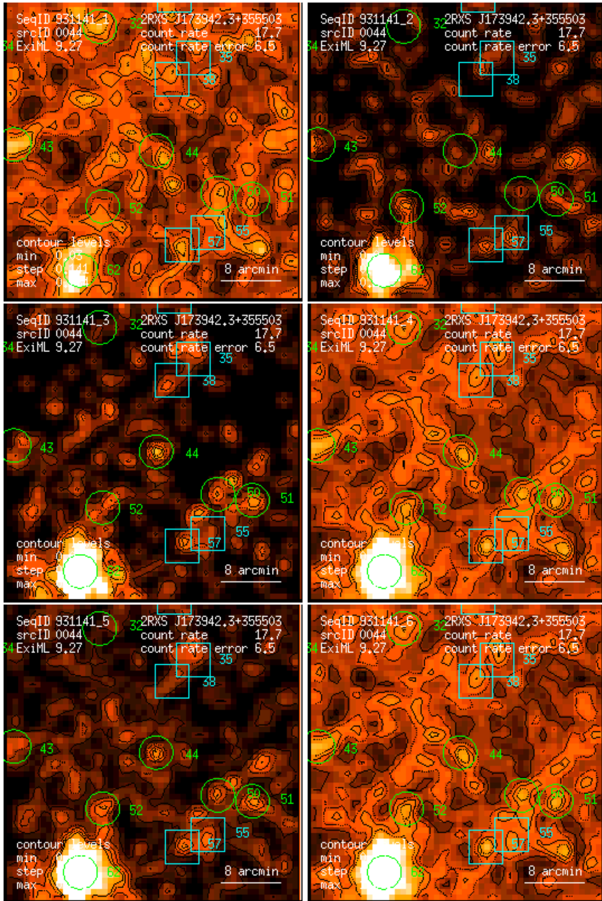
Figure 44: RASS 931141: detection 0044: band rate images, Gaussian filter: (1) PSPC channels 11 – 41, (2) 52 – 90, (3) 91 – 201, (4) 11 – 235, (5) 52 – 201, (6) 11 – 201. Broad band rates in counts/ks. Band rate contour levels in counts/ks/arcmin 2 .
