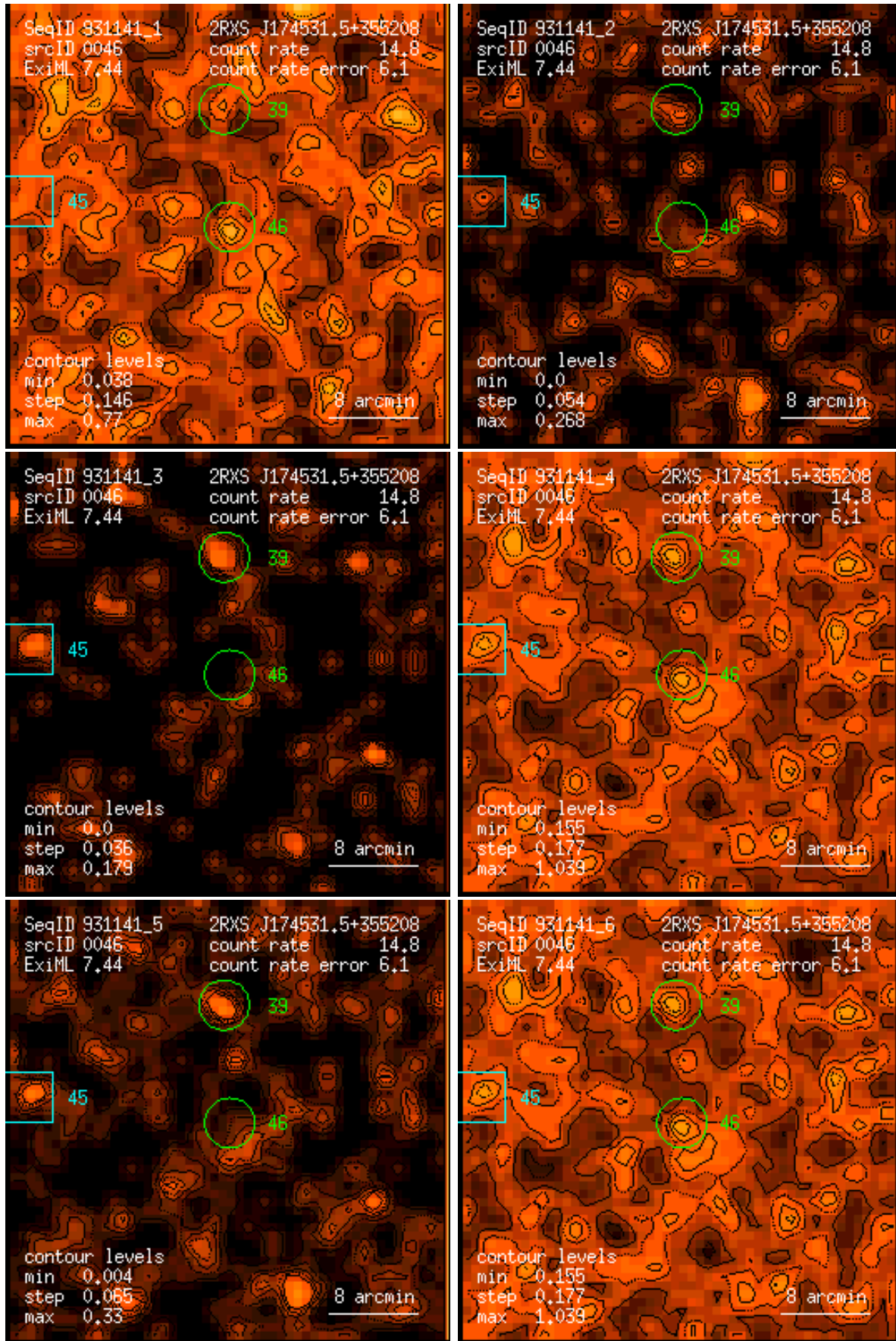
Figure 46: RASS 931141: detection 0046: band rate images, Gaussian filter: (1) PSPC channels 11 – 41, (2) 52 – 90, (3) 91 – 201, (4) 11 – 235, (5) 52 – 201, (6) 11 – 201. Broad band rates in counts/ks. Band rate contour levels in counts/ks/arcmin 2 .
