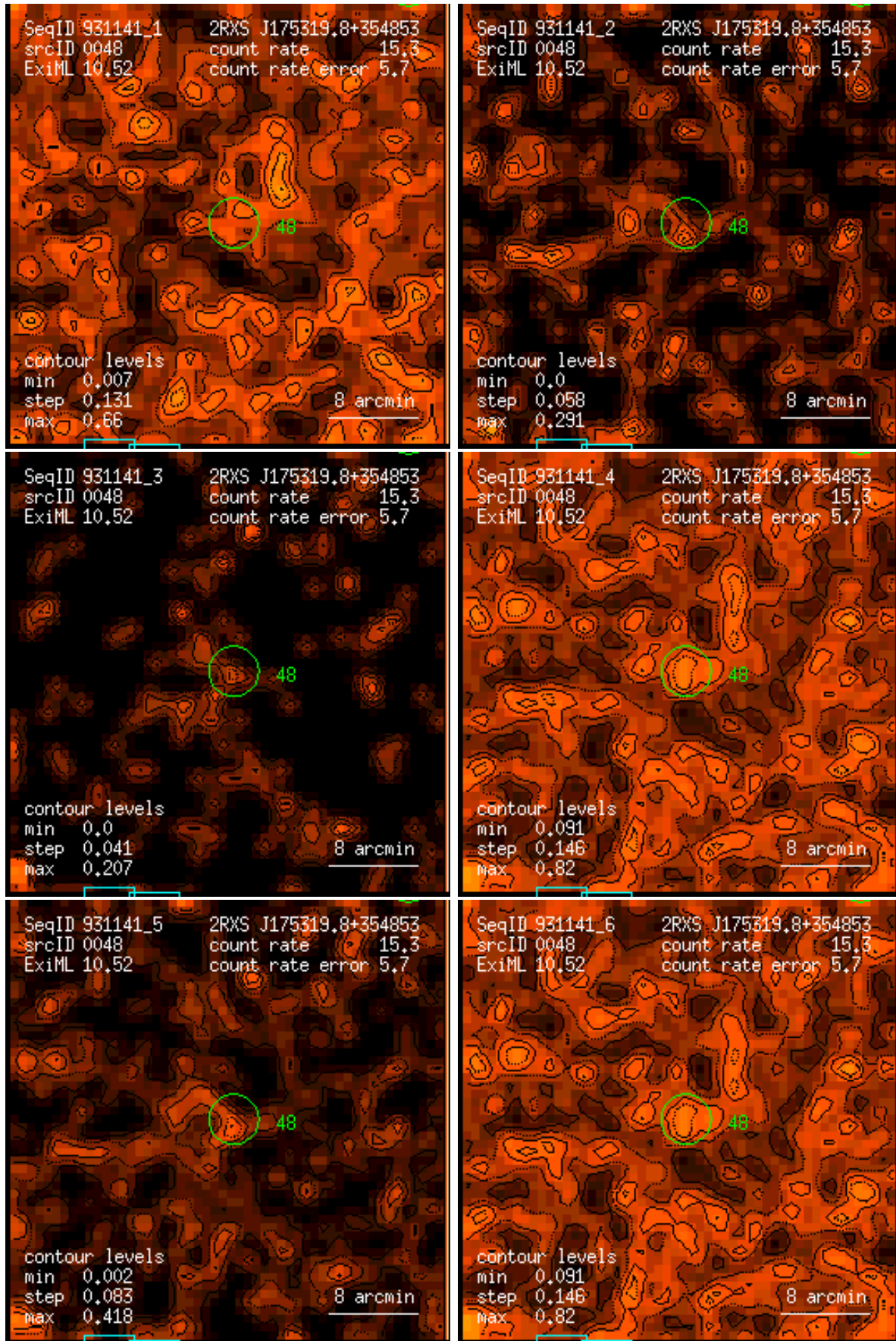
Figure 48: RASS 931141: detection 0048: band rate images, Gaussian filter: (1) PSPC channels 11 – 41, (2) 52 – 90, (3) 91 – 201, (4) 11 – 235, (5) 52 – 201, (6) 11 – 201. Broad band rates in counts/ks. Band rate contour levels in counts/ks/arcmin 2 .
